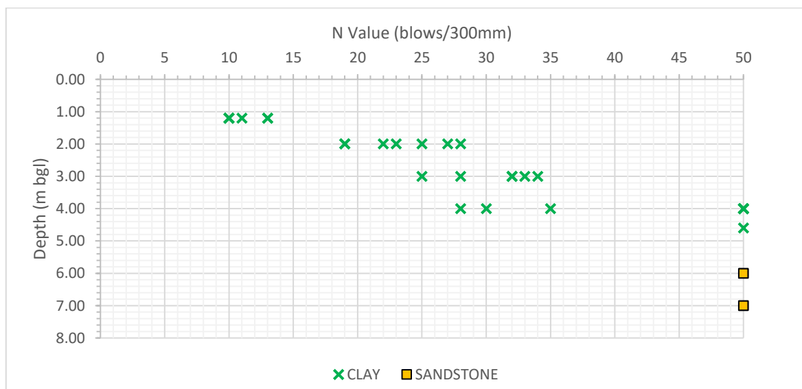
Figure 4: SPT Results
