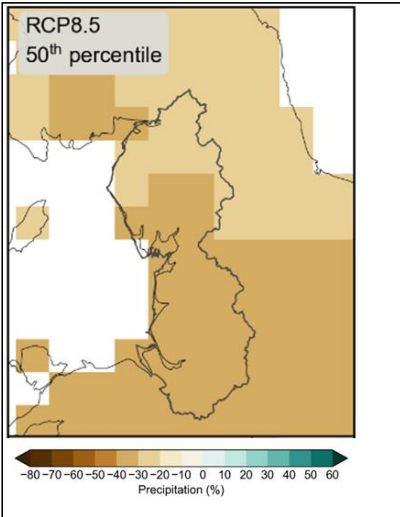
Figure 7.2 Summer precipitation anomaly in North West England for 2080-2099 minus 1981-2000.
