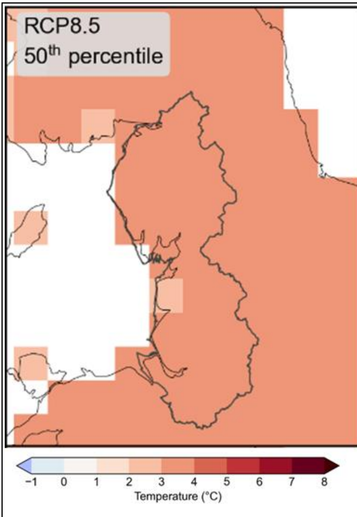
Figure 7.3 Winter mean temperature anomaly in North West England for 2080-2099 minus 1981-2000.
