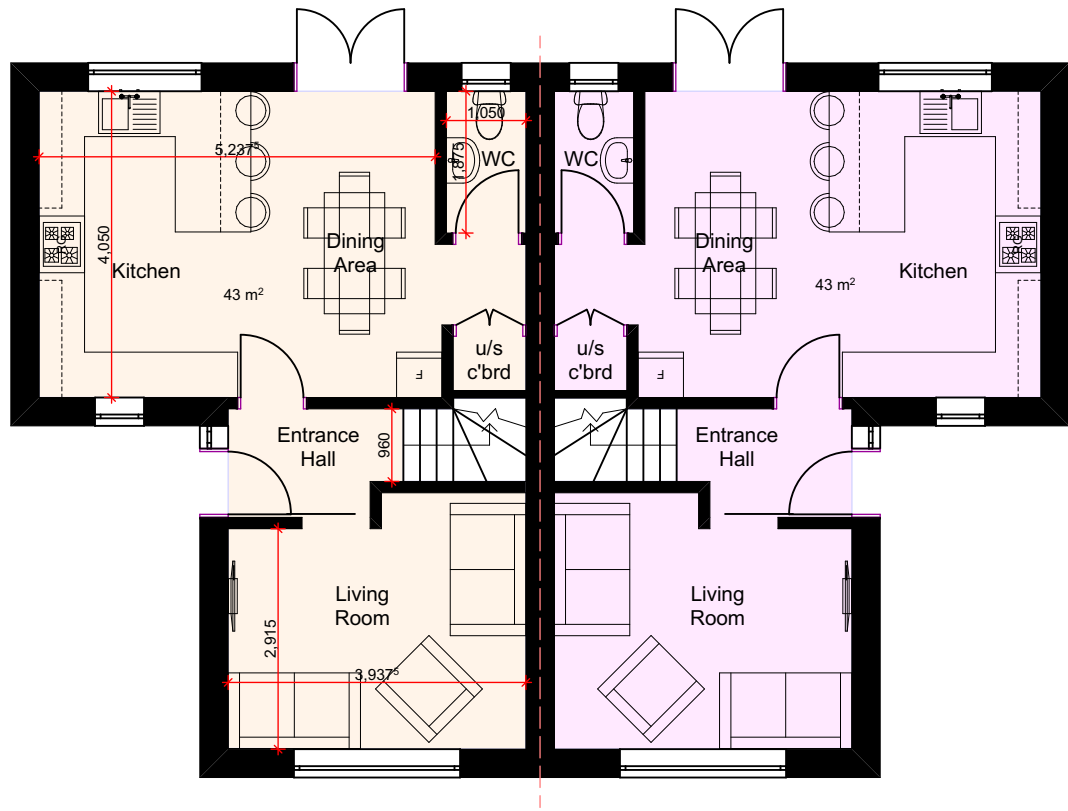
PROPOSED GA GROUND FLOOR PLAN UNITS 2-7
