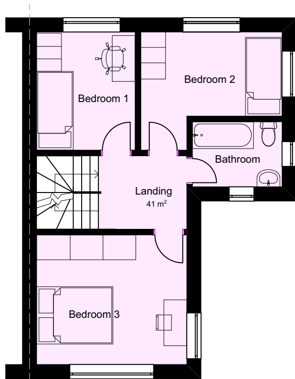
PROPOSED GA FIRST FLOOR PLAN UNITS 8
