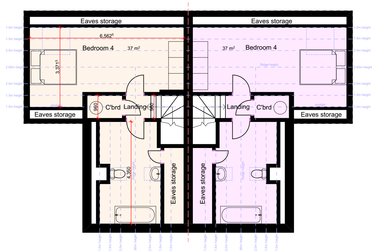
PROPOSED GA SECOND FLOOR PLAN UNITS 1- 8
