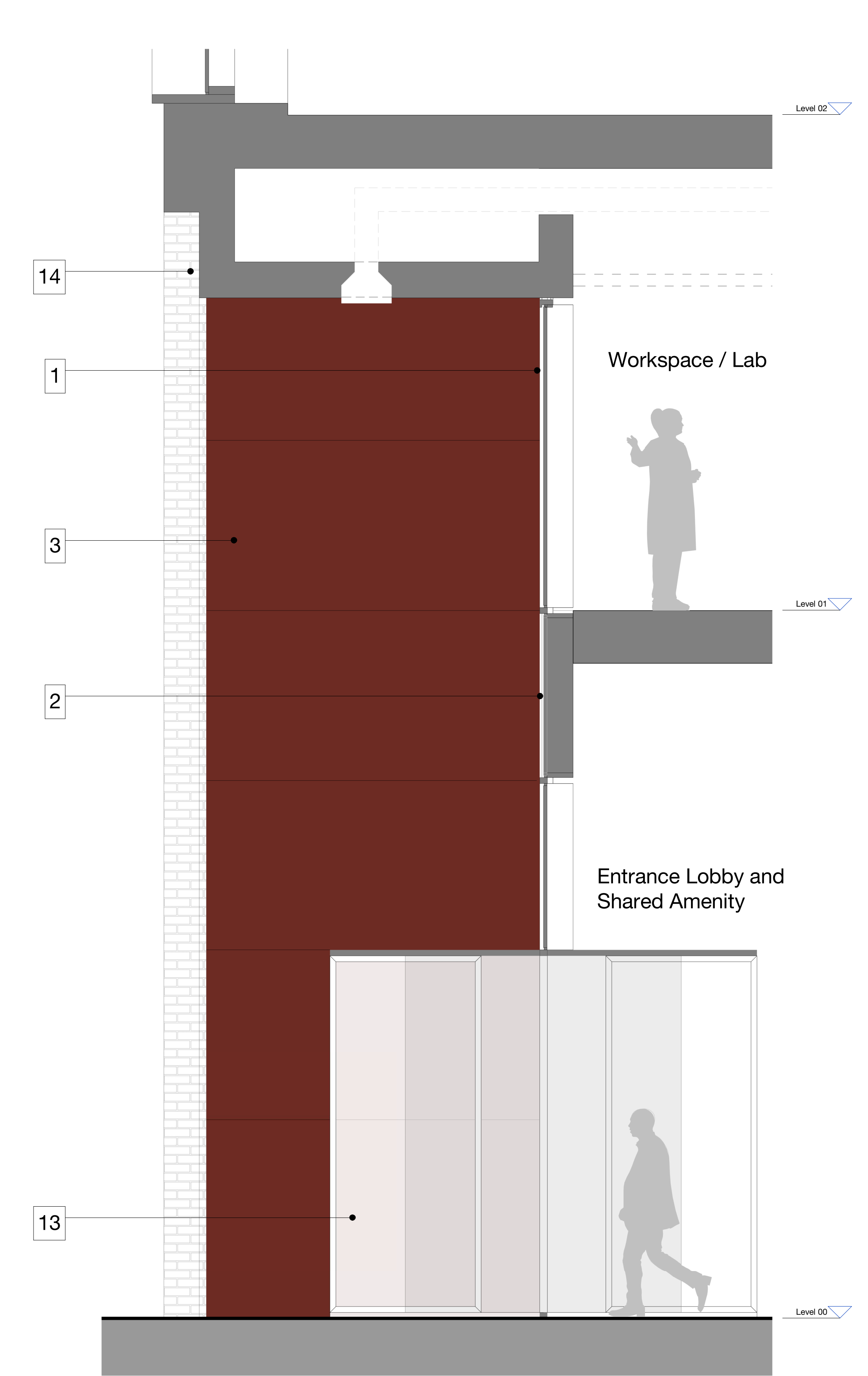
2 Proposed B1 - Base Section
