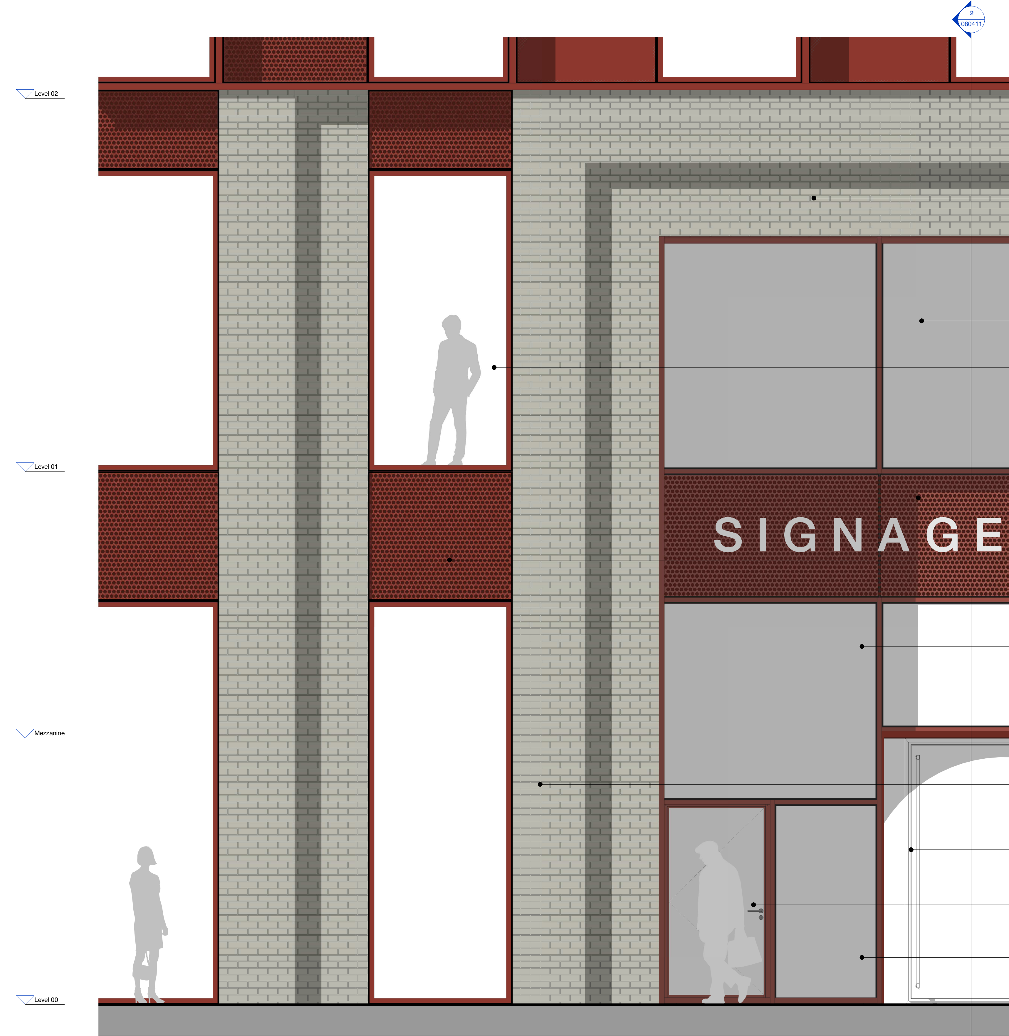
1 Proposed B1 - Base Elevation
