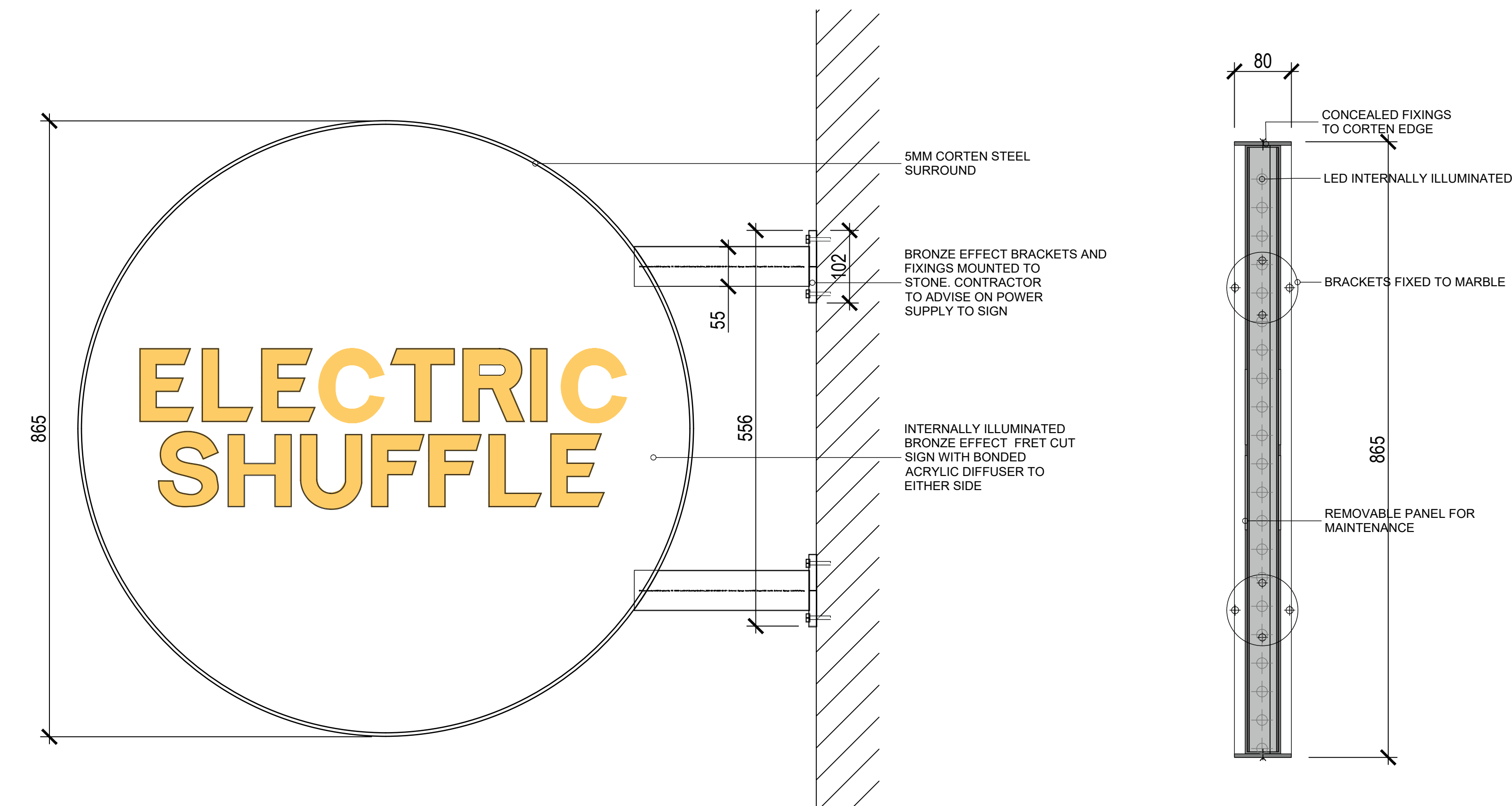
Proposed Wall-Mounted Signage Detail Scale 1:5
