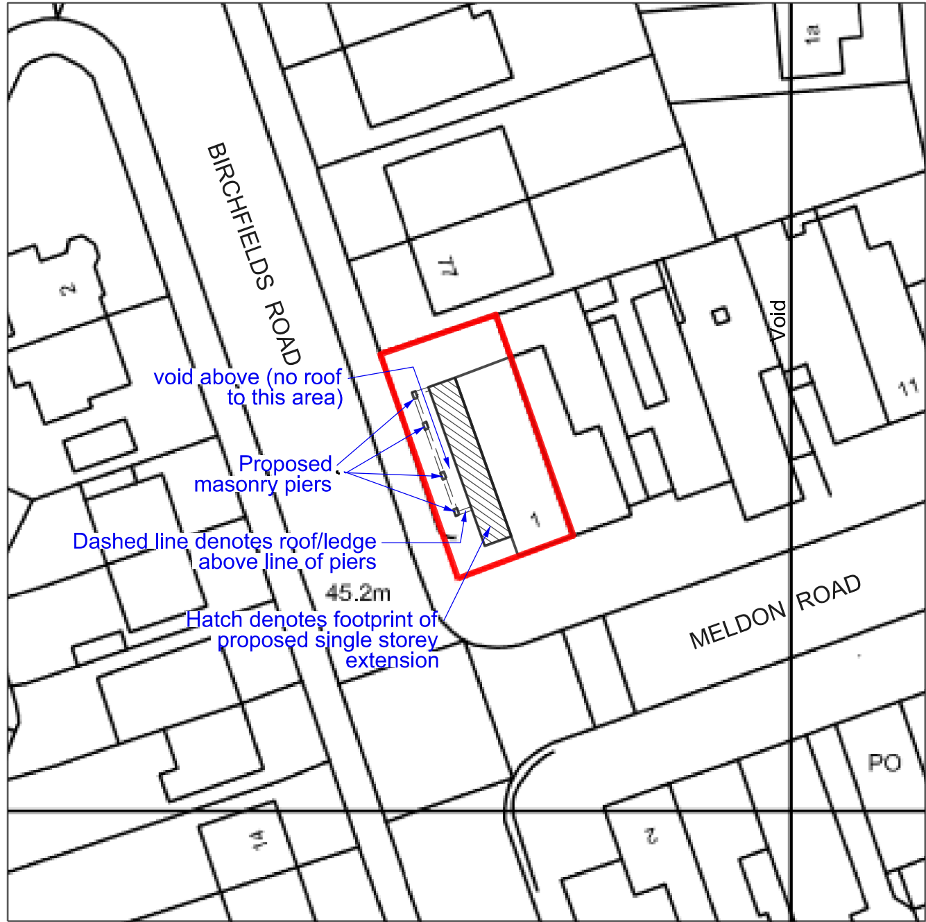
Block Plan 1:500
