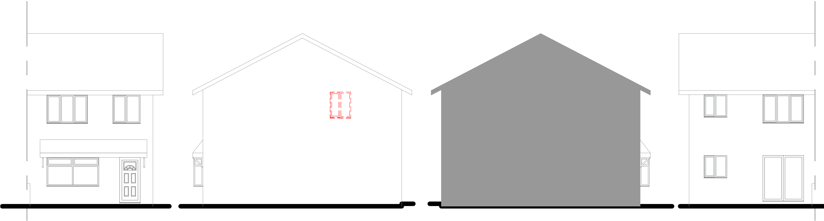
Front Elevation
