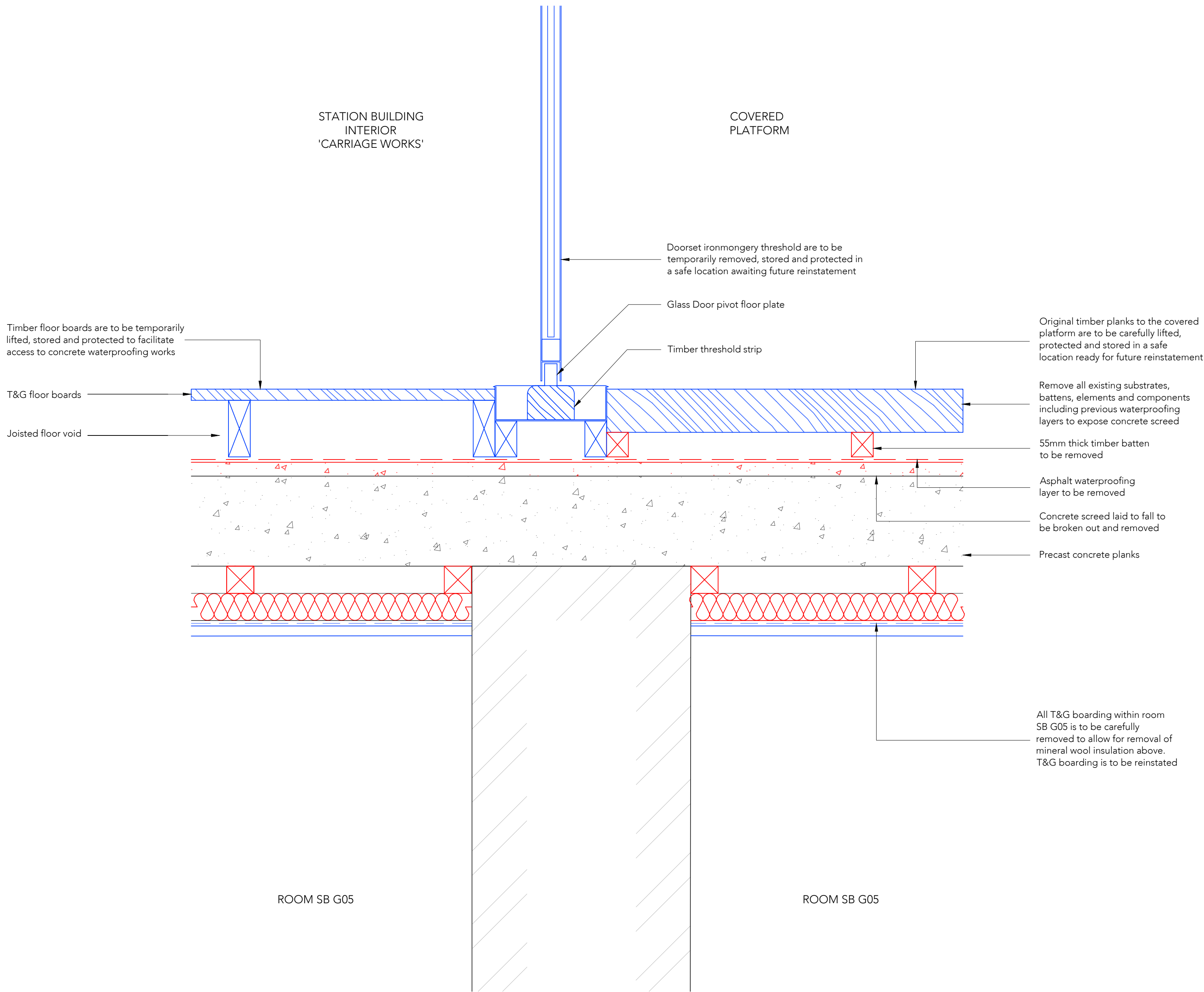
Typical Detail Through Glass Door Threshold K-K Demolition & Removals Scale 1:5
