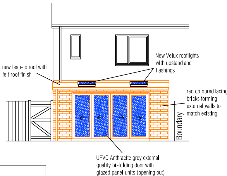
Proposed rear South Elevation, 1:100
