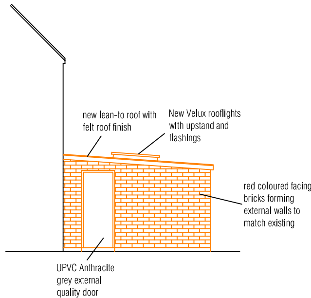
Proposed side east Elevation, 1:100
