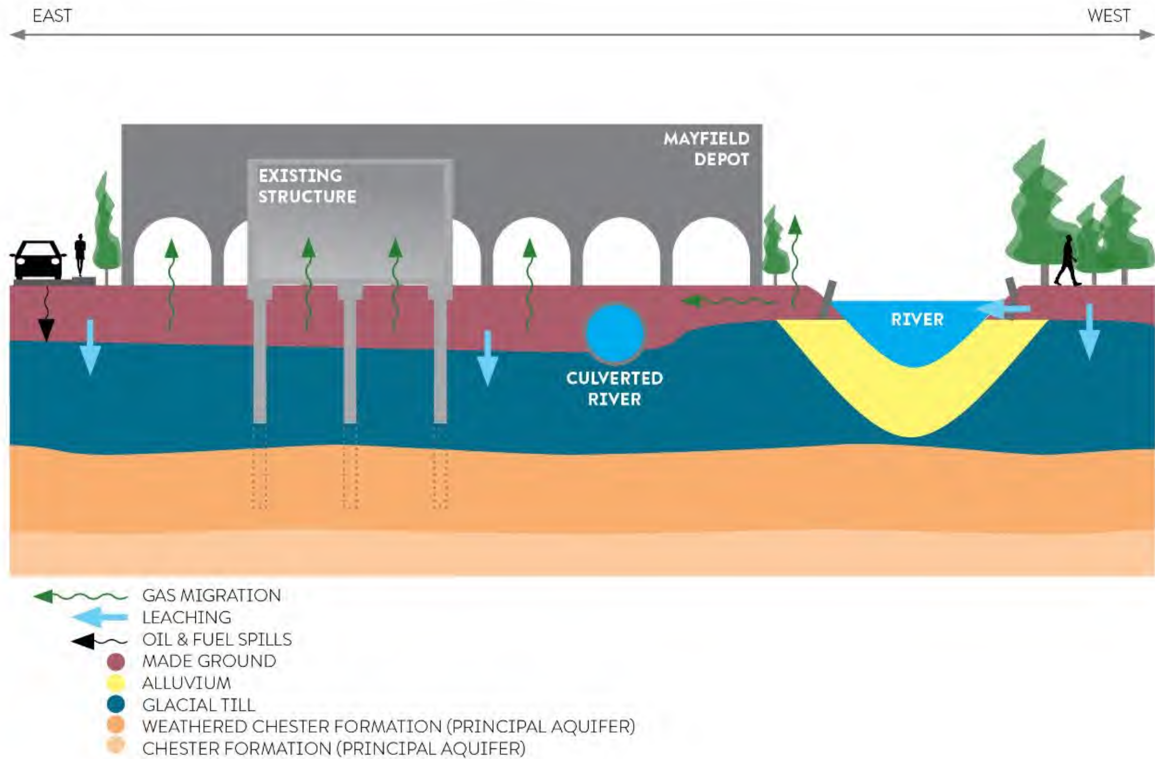
Figure: 10.2 Title: Pre-Construction Conceptual Site Model Project: Mayfield Phase 1 Date: September 2019 Scale: NTS
