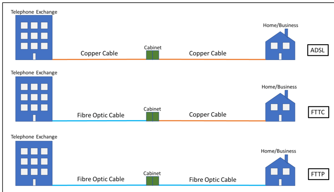
Figure 4 – Common types of broadband (fixed line)
