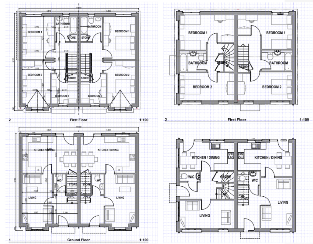
Figure 2 – Floor Plans
