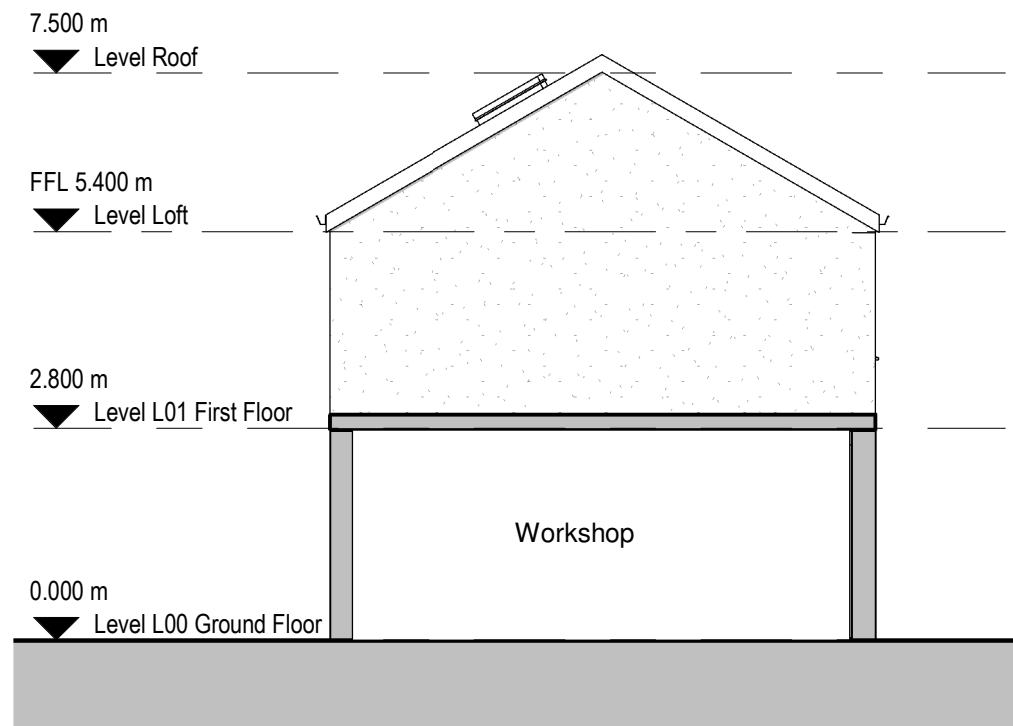
4 Proposed South Elevation 1 : 100
