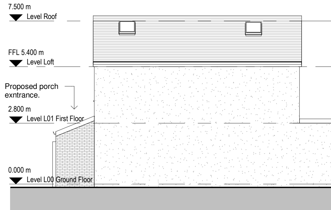
3 Proposed West Elevation 1 : 100
