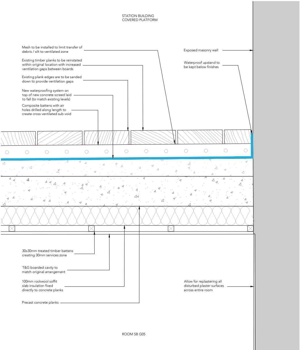
Station House External Wall/Floor Junction Detail as Proposed Scale 1:10
