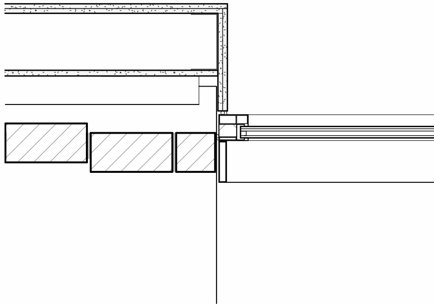
1 Sample Panel Plan Detail 1 : 10
