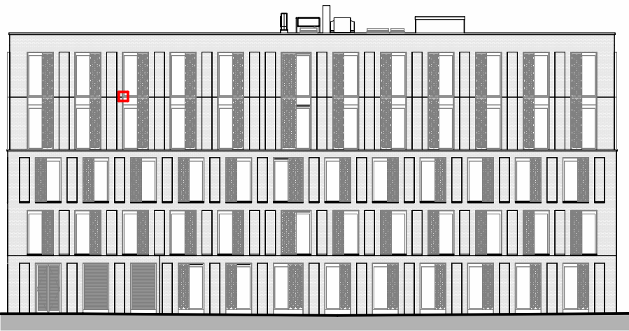
Key North Elevation
