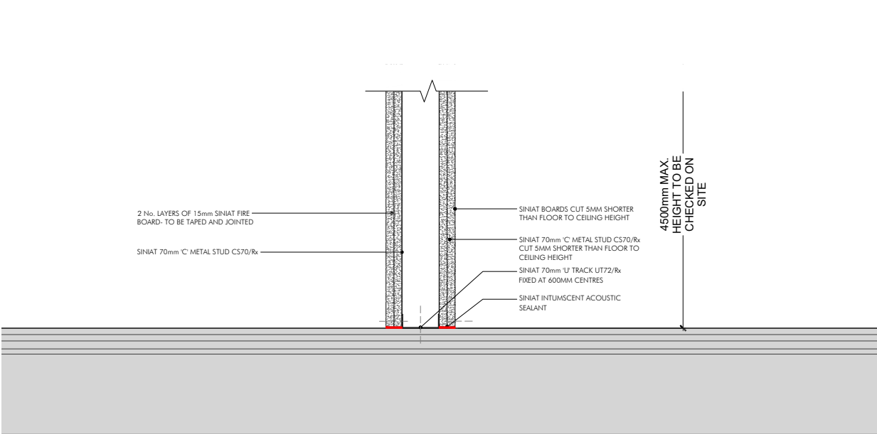
TYPICAL PARTITION 'TYPE E' SECTION ALIGNED WITH BRICK ARCHES SINIAT REFERENCE CS70R-215F SCALE 1:5
