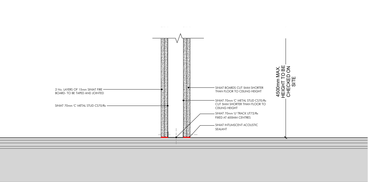
TYPICAL PARTITION 'TYPE E' SECTION PERPENDICULAR TO BRICK ARCHES SINIAT REFERENCE CS70R-215F SCALE 1:5
