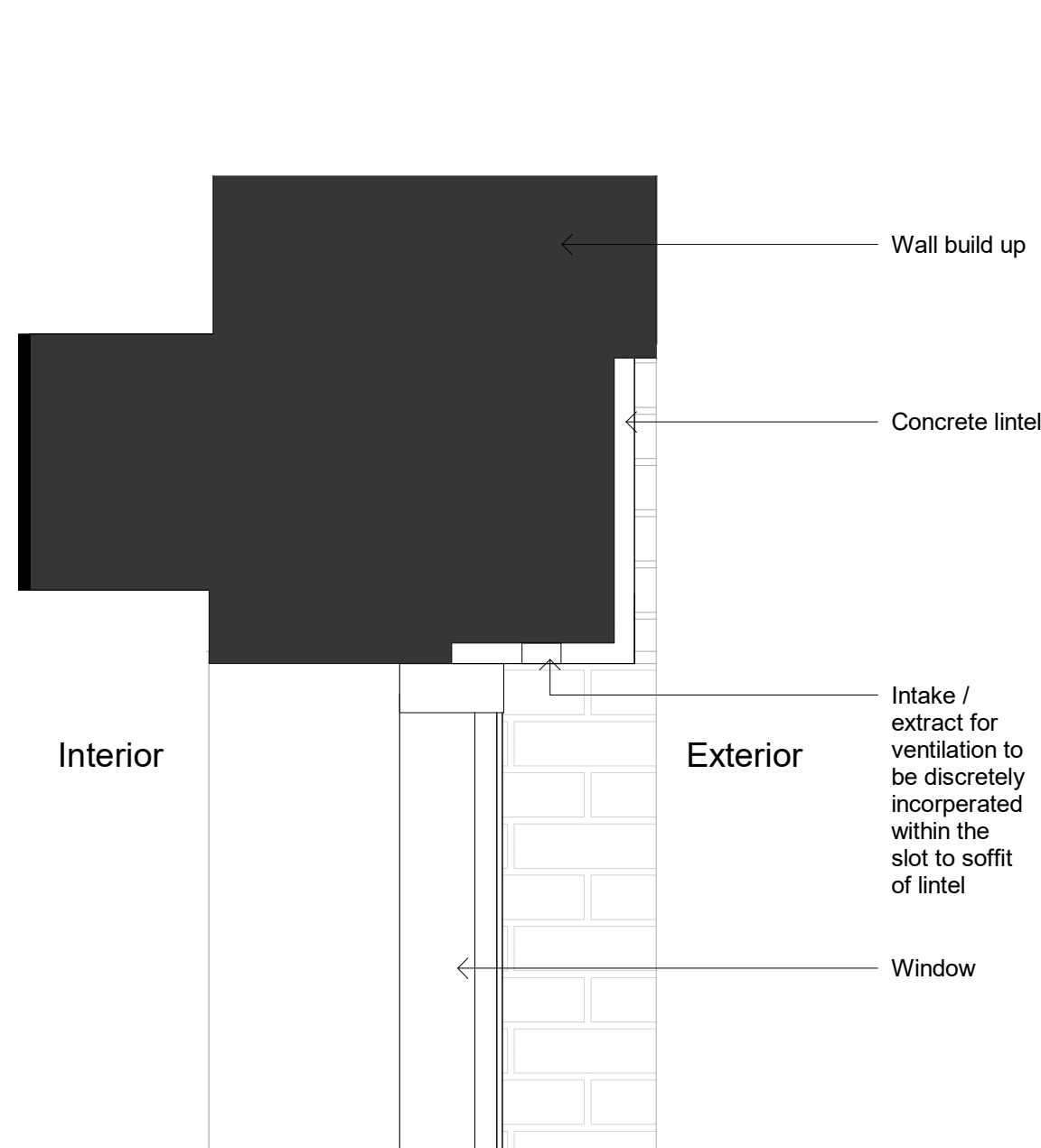
Typical Lintel Detail 1 : 10
