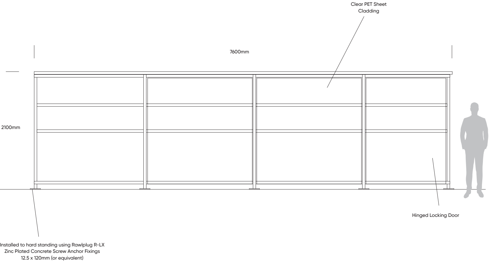
FACE VIEW
