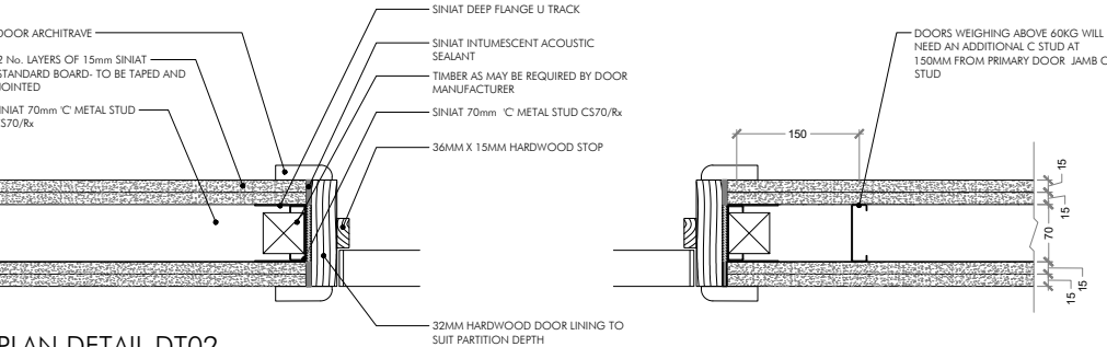
PLAN DETAIL DT02 TYPICAL PARTITION 'TYPE A' DOOR JAMB DETAIL (NON FIRE RATED) SINIAT REFERENCE CS70R-215S† SCALE 1:5
