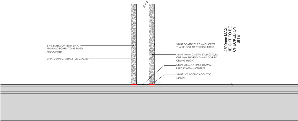
TYPICAL PARTITION 'TYPE A' SECTION ALIGNED WITH BRICK ARCHES SINIAT REFERENCE CS70R-215S† SCALE 1:5
