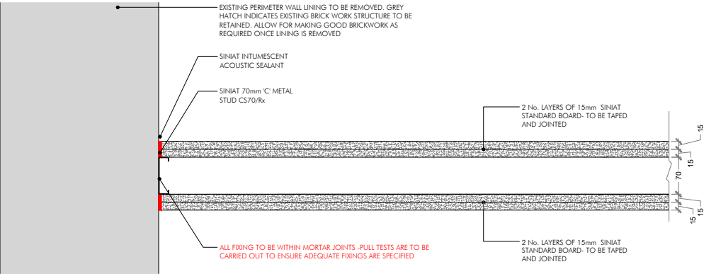
PLAN DETAIL DT01 TYPICAL PARTITION 'TYPE A' ABUTMENT WITH EXISTING WALL SINIAT REFERENCE CS70R-215S† SCALE 1:5
