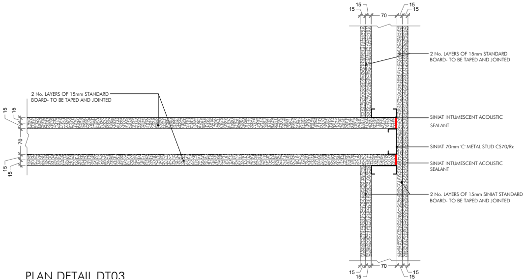
PLAN DETAIL DT03 TYPICAL PARTITION 'TYPE A' T JUNCTION SINIAT REFERENCE CS70R-215S† SCALE 1:5
