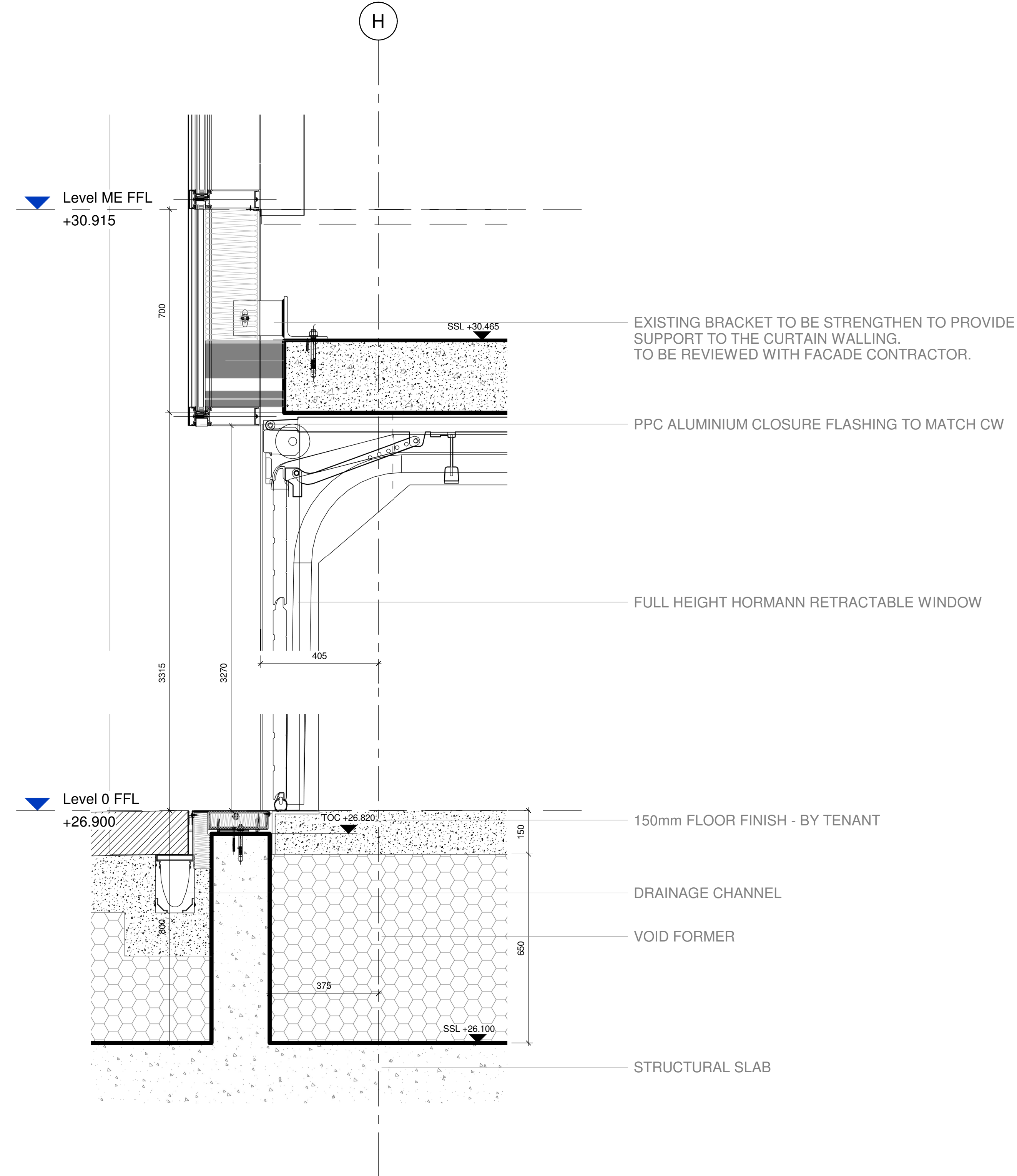
02 RETRACTABLE WINDOW - PROPOSED SECTION 1 : 10 Referenced by 03 / 22900
