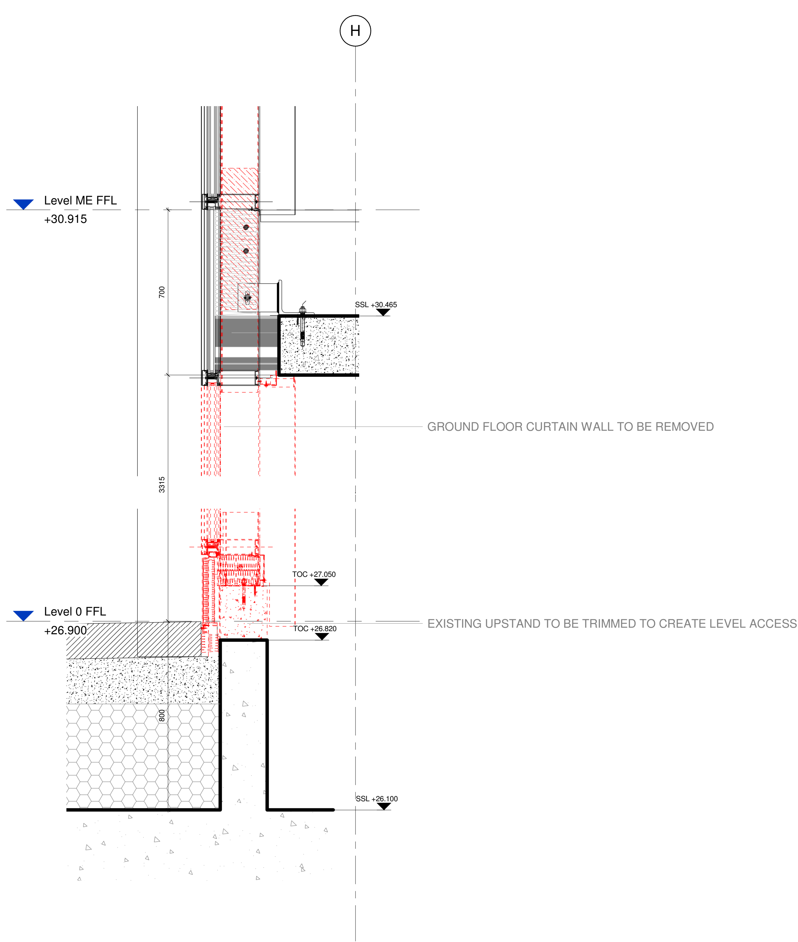
01 RETRACTABLE WINDOW - EXISTING SECTION 1 : 10 Referenced by 02 / 22900
