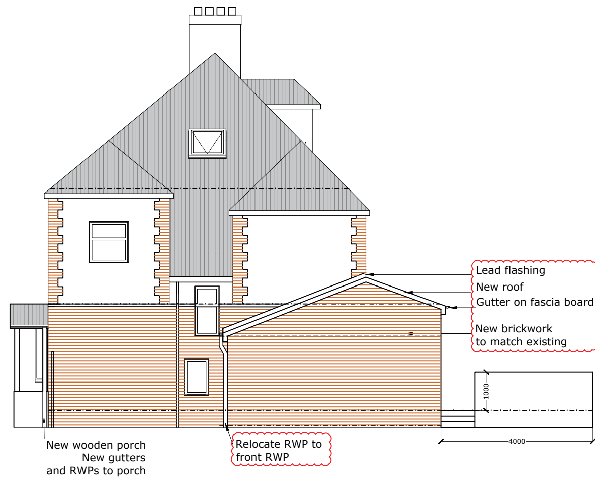
SIDE ELEVATION
