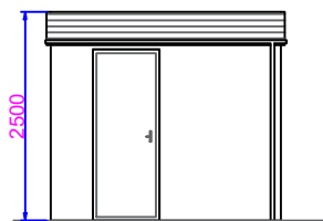
Side Elevation
