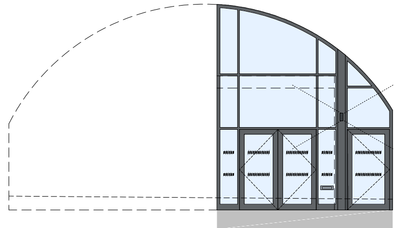
ARCH 10 ELEVATION TO RECESSED FRONTAGE
