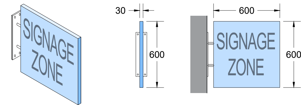
TYPICAL FIN SIGNAGE
