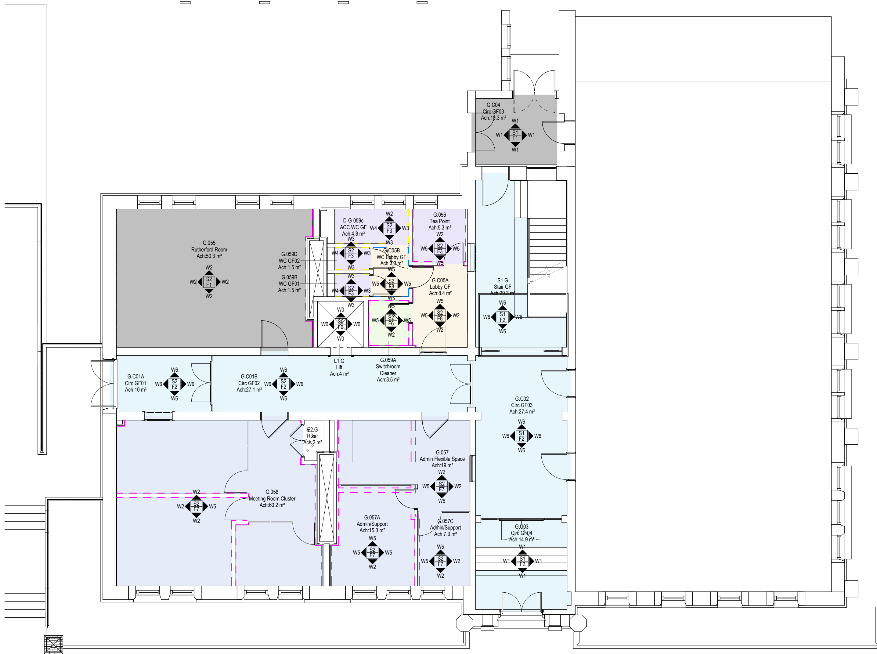
1 Proposed Finishes GA Plan_Level 00 1 : 100
