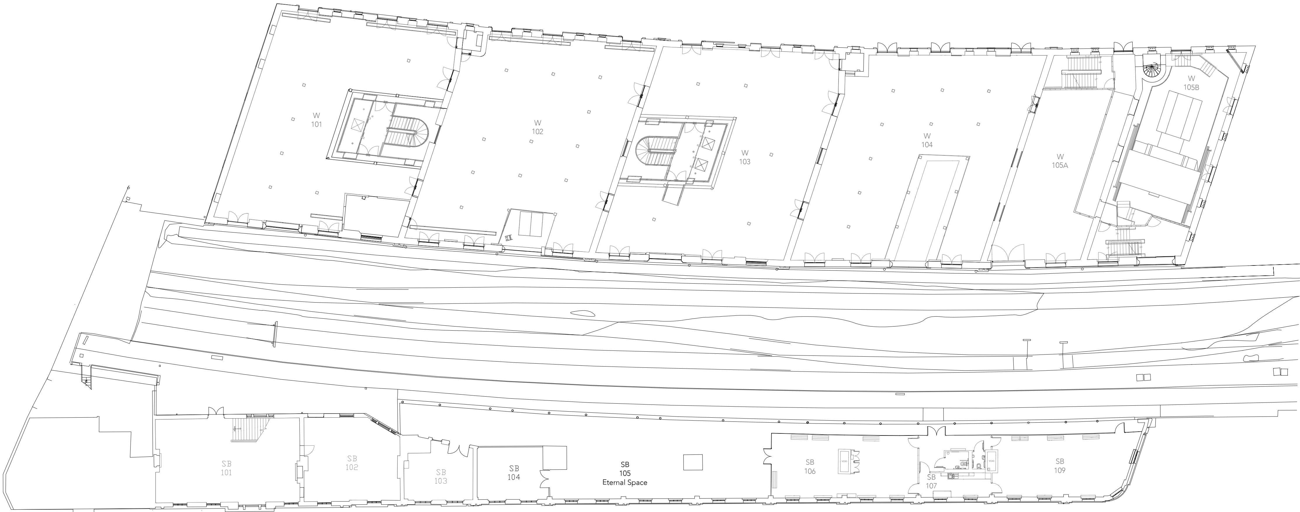
First Floor / Track Level Plan As Existing - 1830's Warehouse, Viaduct and Station Building Scale 1:200
