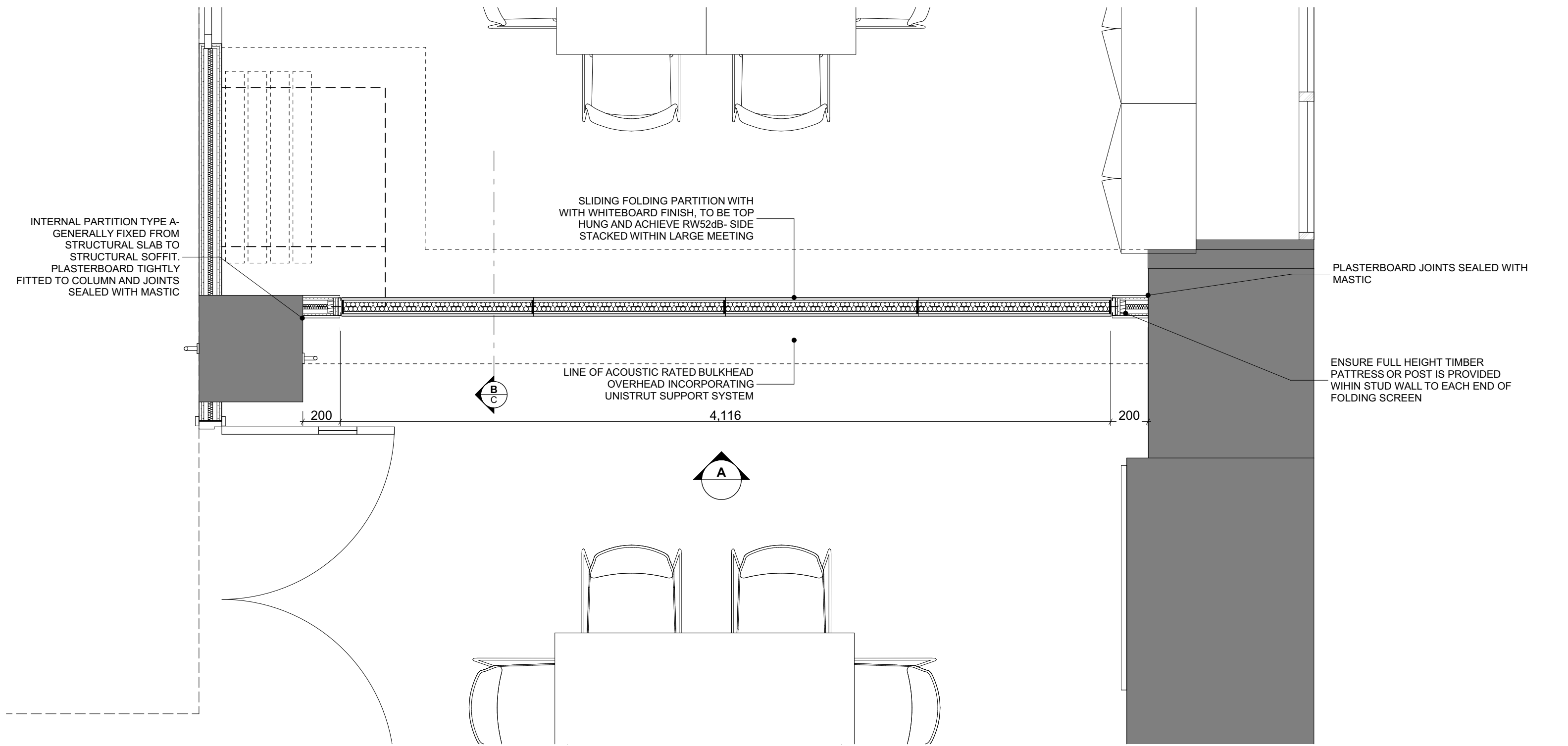
FOLDING PARTITION PLAN 1:20
