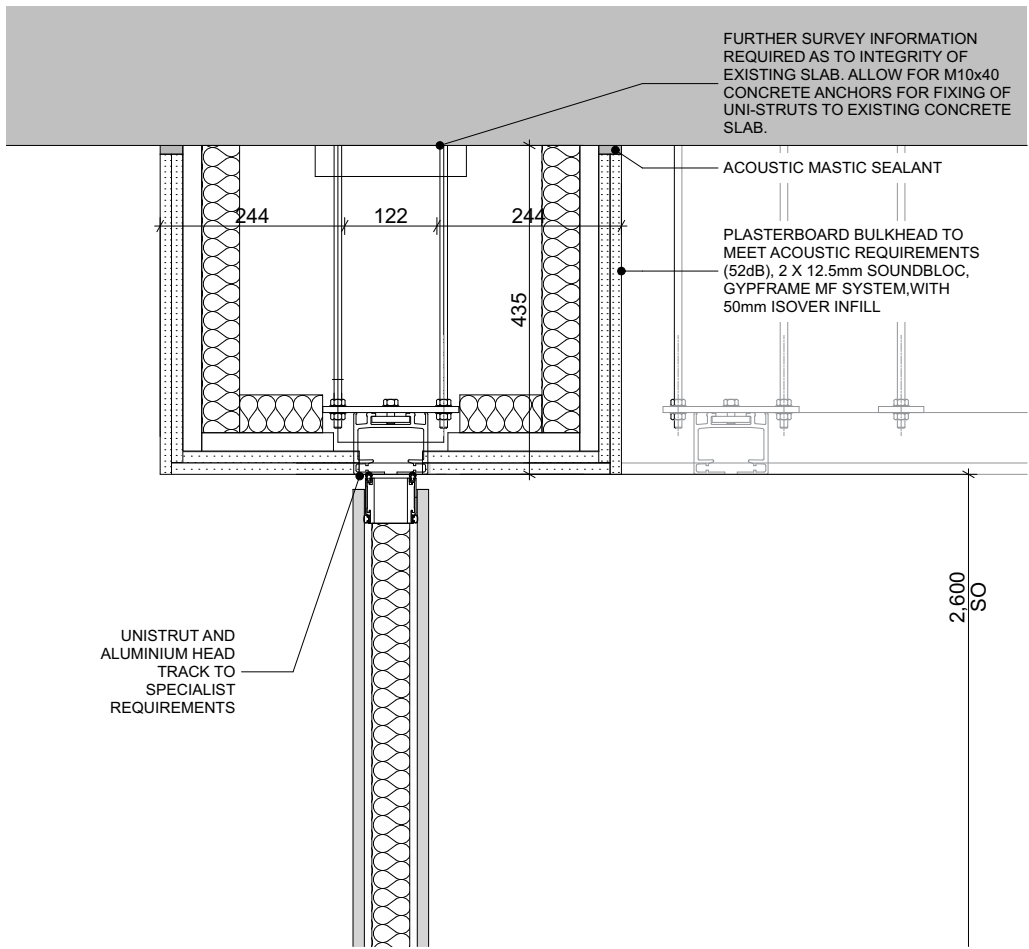
DETAIL B: TYPICAL FOLDING PARTITION HEAD TRACK 1:10
