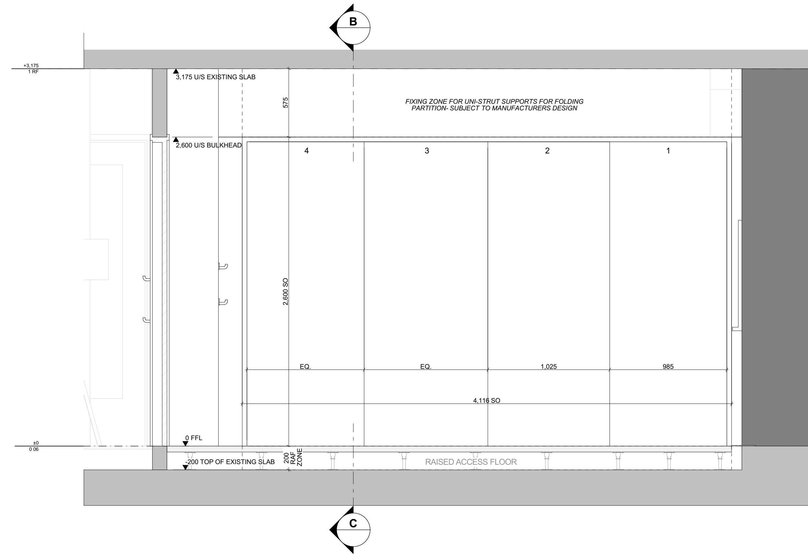
ELEVATION A: FOLDING PARTITION 1:20
