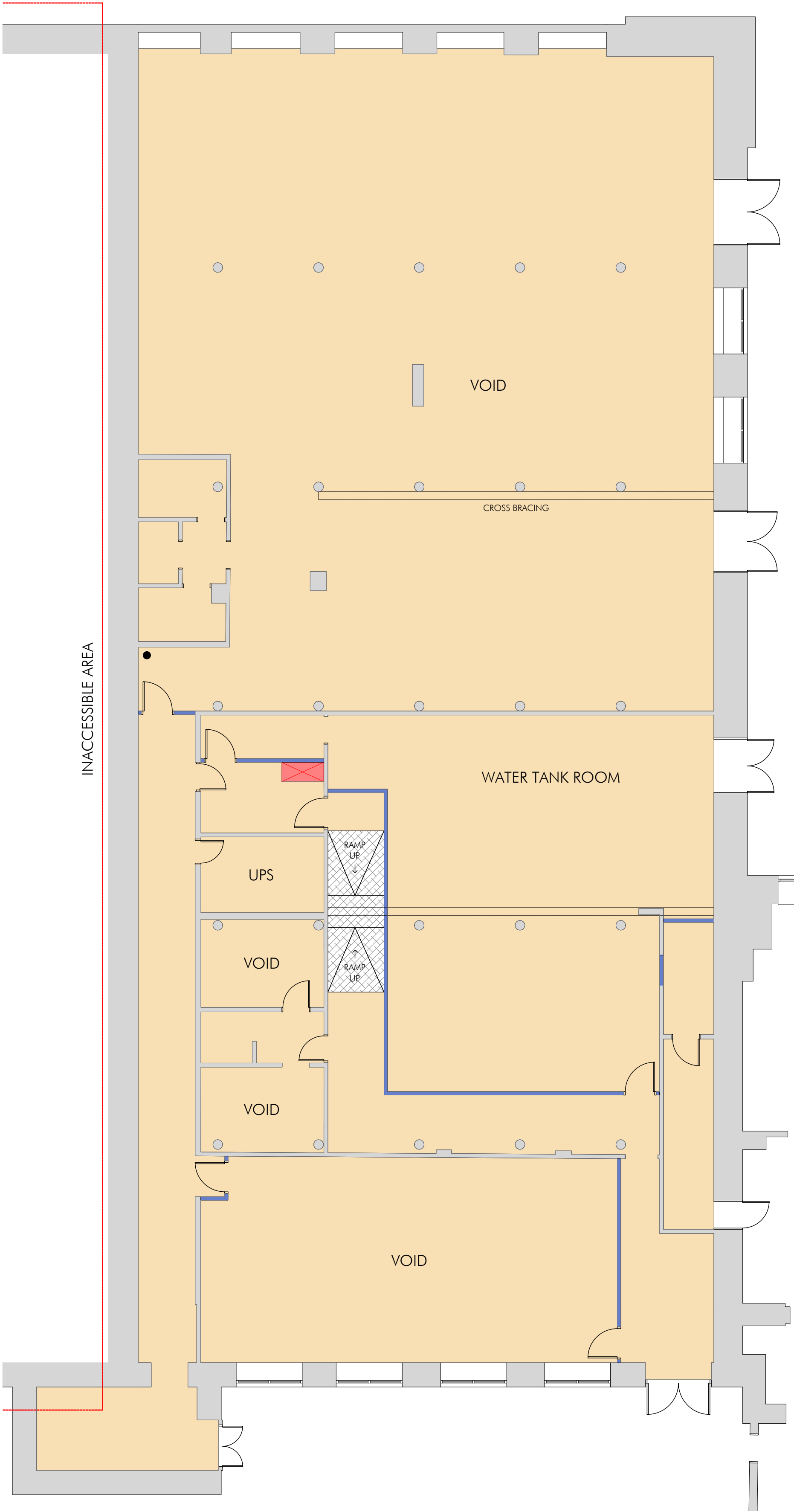
PROPOSED BASEMENT FLOOR FINISHES PLAN
