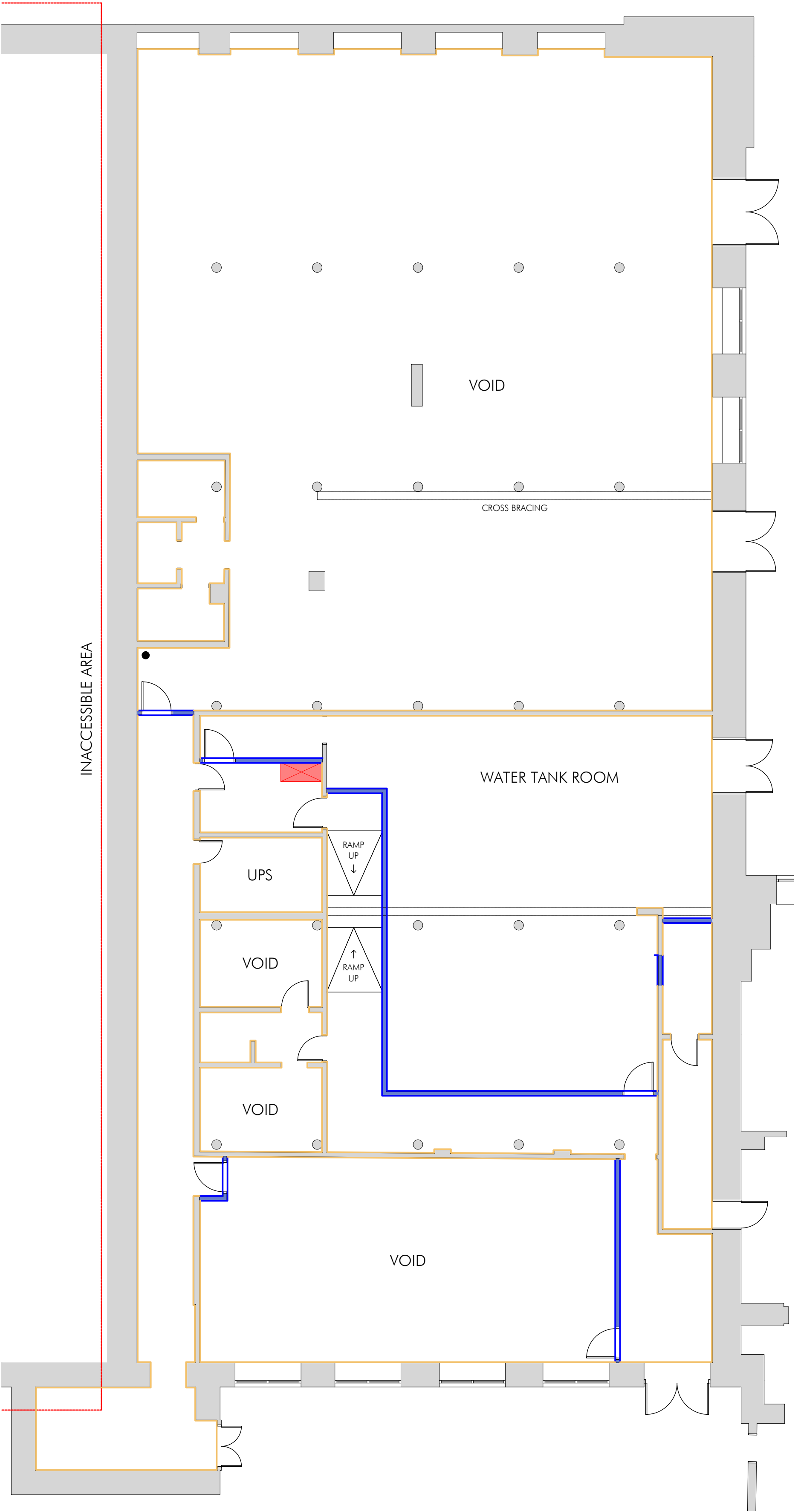
PROPOSED BASEMENT FLOOR WALL AND STRUCTURE FINISHES PLAN
