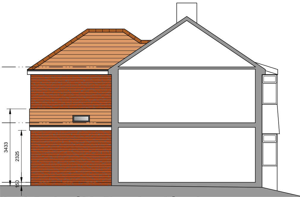
North Facing Side Elevational Section
