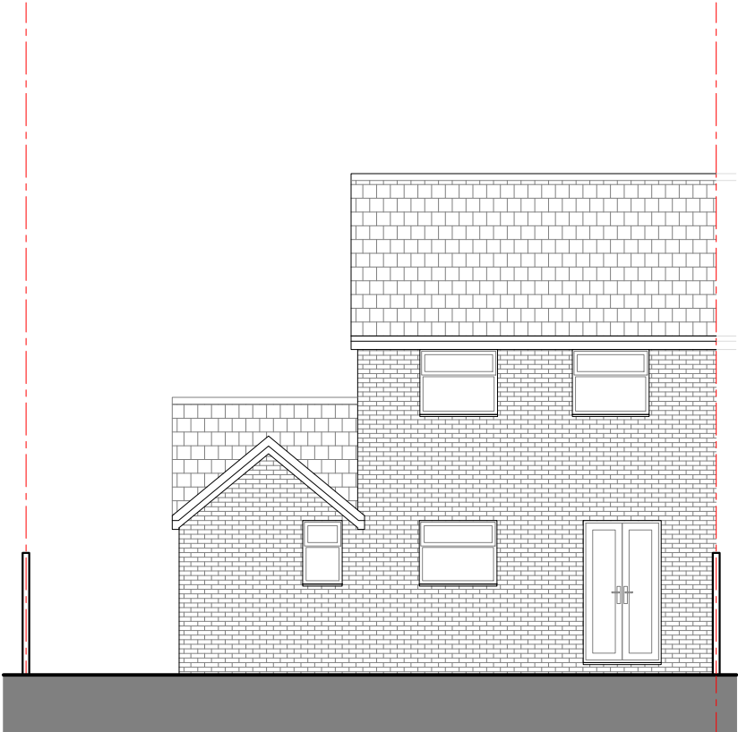
EXISTING REAR ELEVATION 1:100 @ A3
