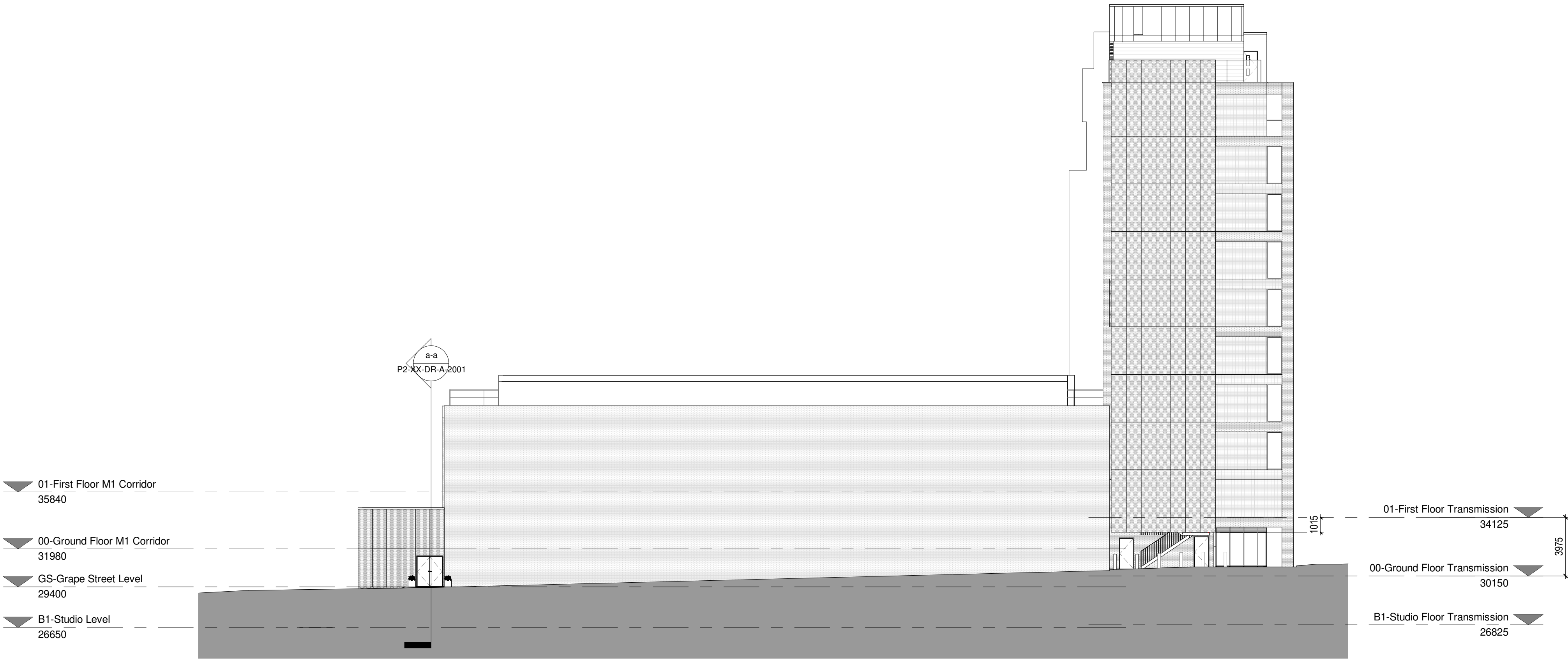
Proposed Grape Street Elevation - Stair 7 1 : 200
