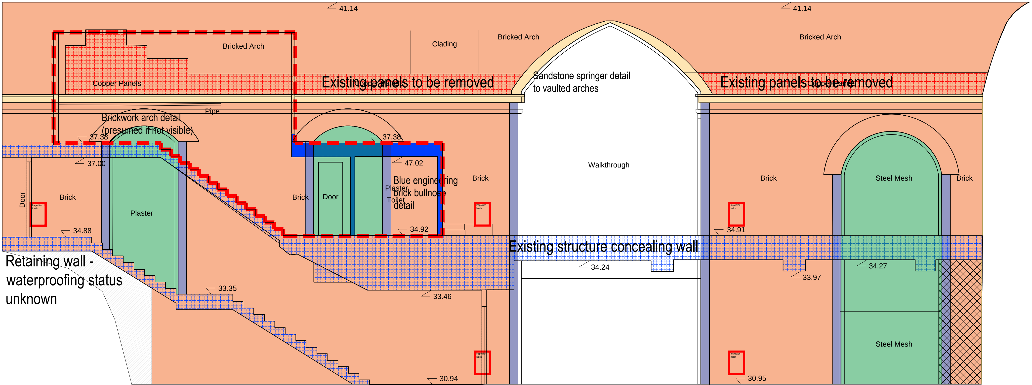
Arch 7 Internal Elevation 2
