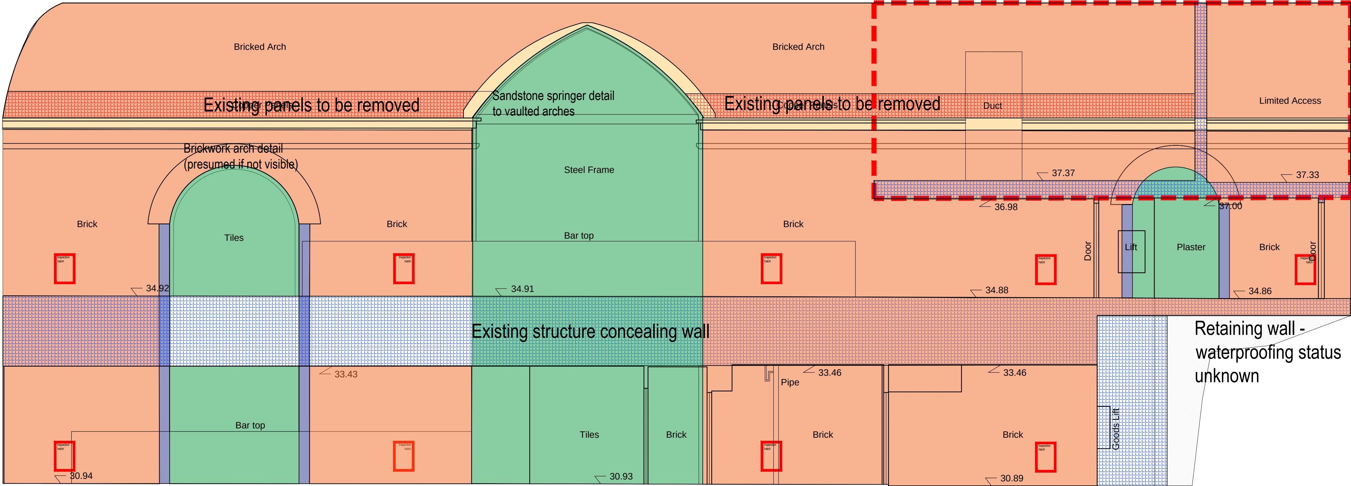
Arch 7 Internal Elevation 1
