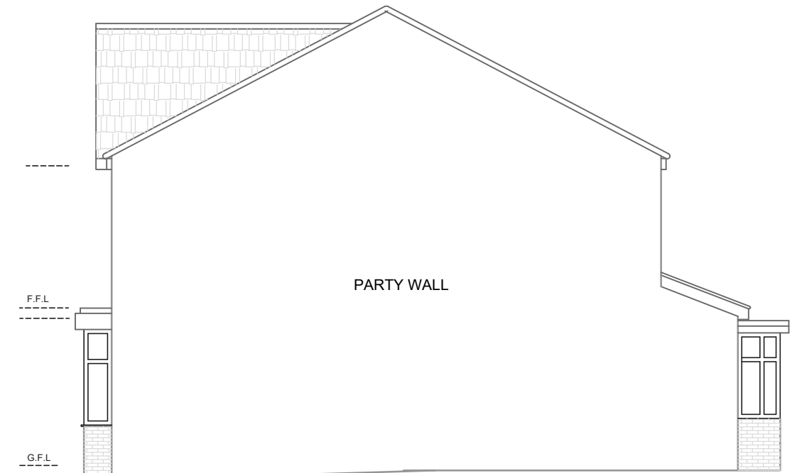
EXISTING SIDE ELEVATION (SOUTH)
