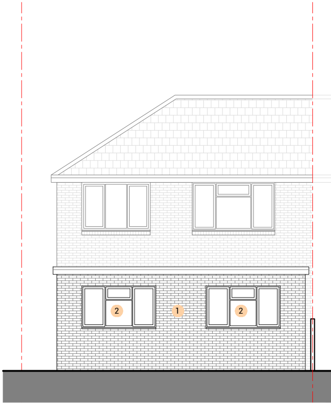
PROPOSED REAR ELEVATION 1:100 @ A3 0m 1m 3m 5m Key 1 Brickwork to match existing 2 PVC Window to match existing 3 PVC Window to match existing (Obscure Glazing)
