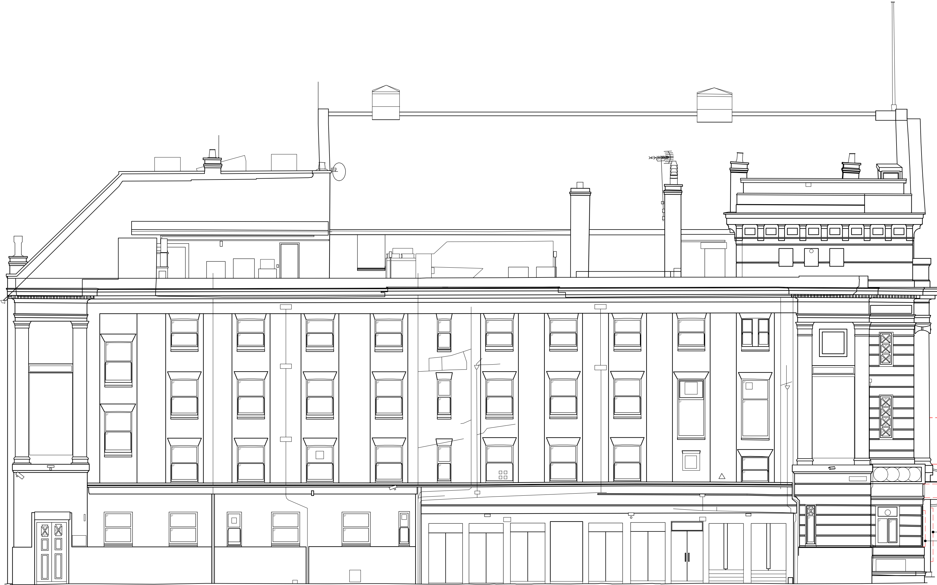
STRIP OUT BYROM STREET ELEVATION 1:100
