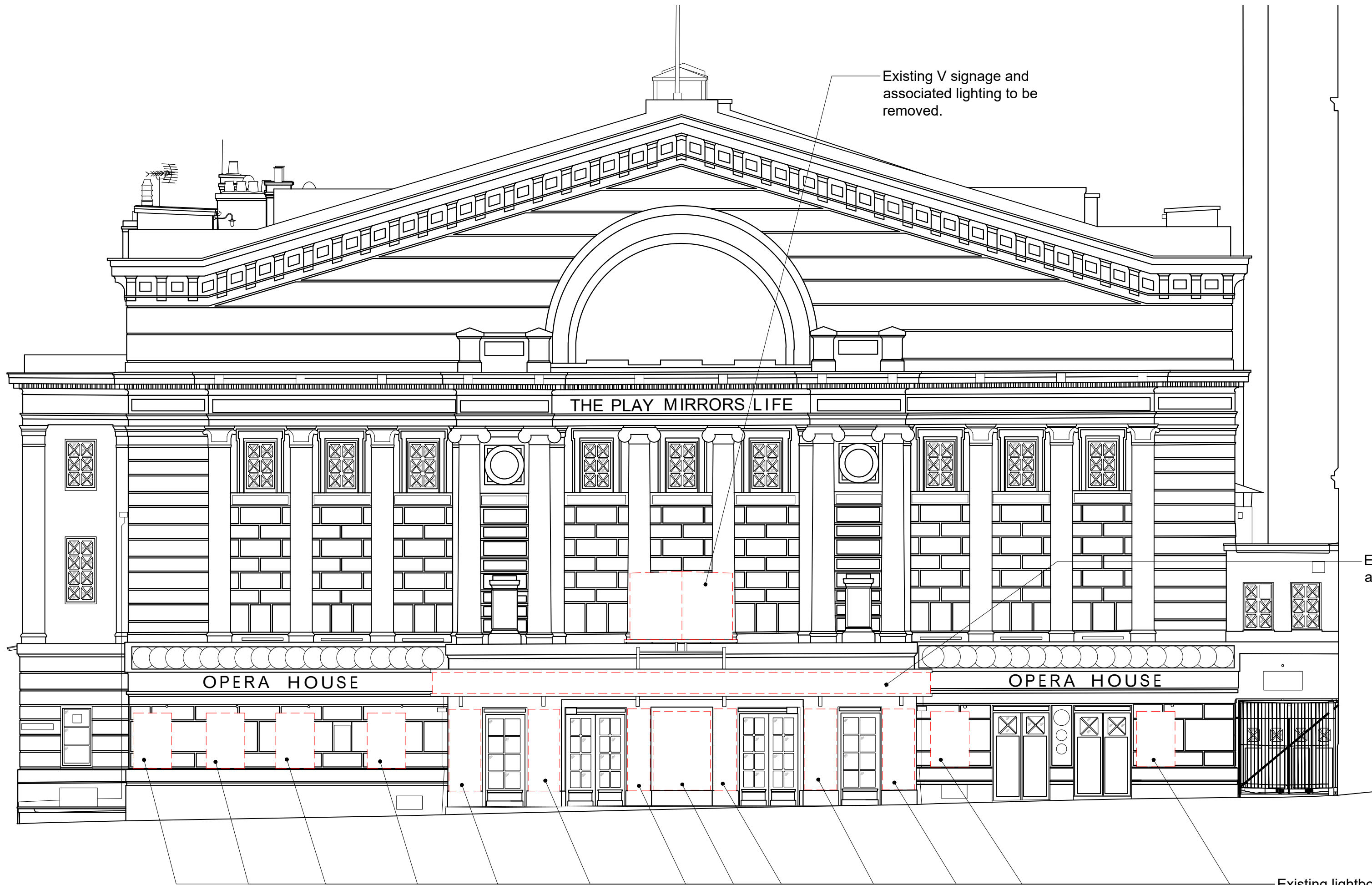
STRIP OUT QUAY STREET ELEVATION 1:100
