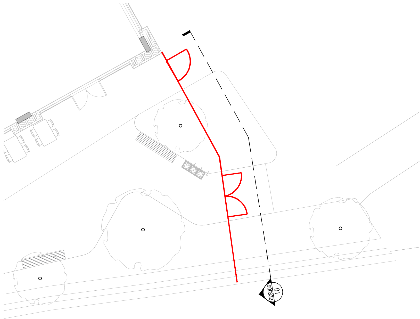
01 900332 B3 - Steel Fenceline and Pedestrian Entrance Access Scale 1: 100 @A1
