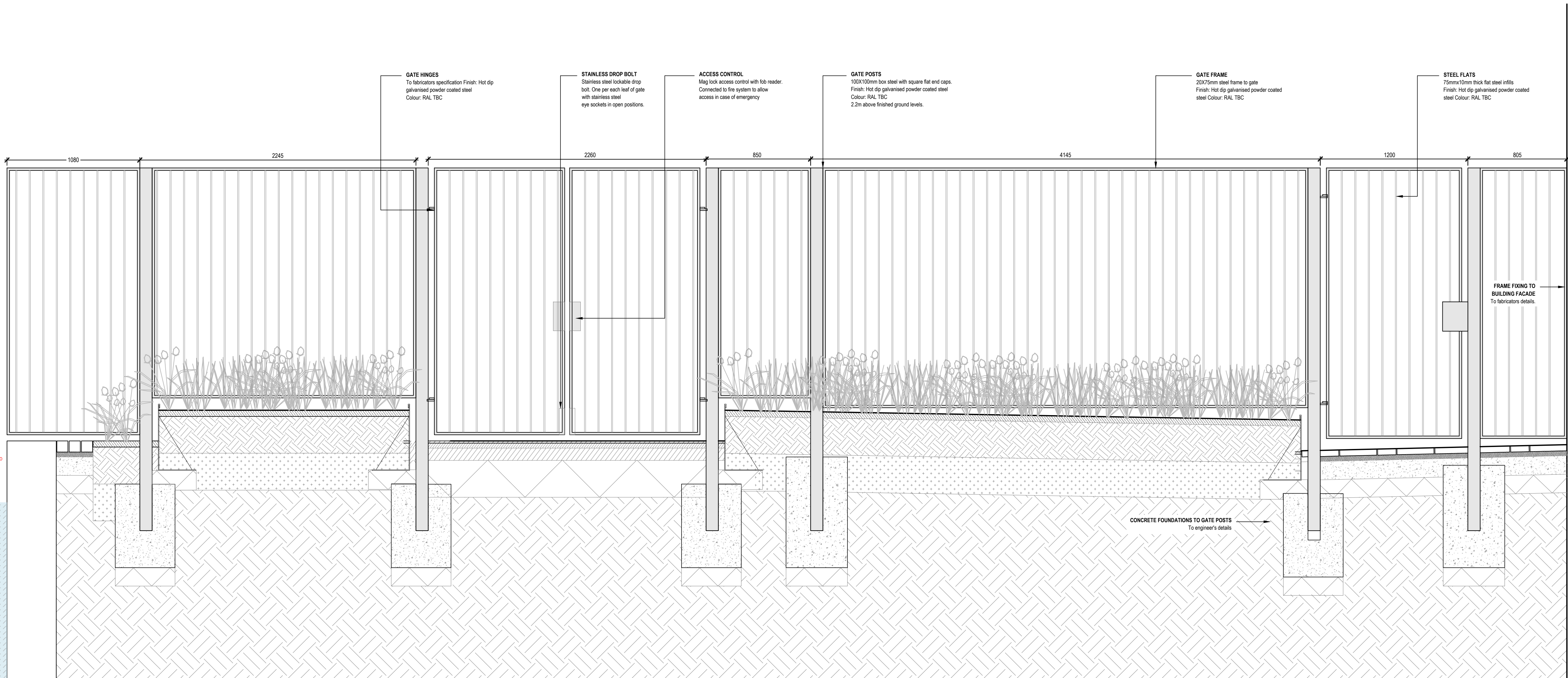
01 900332 B3 - Steel Fenceline and Pedestrian Entrance Access Scale 1: 20 @A1
