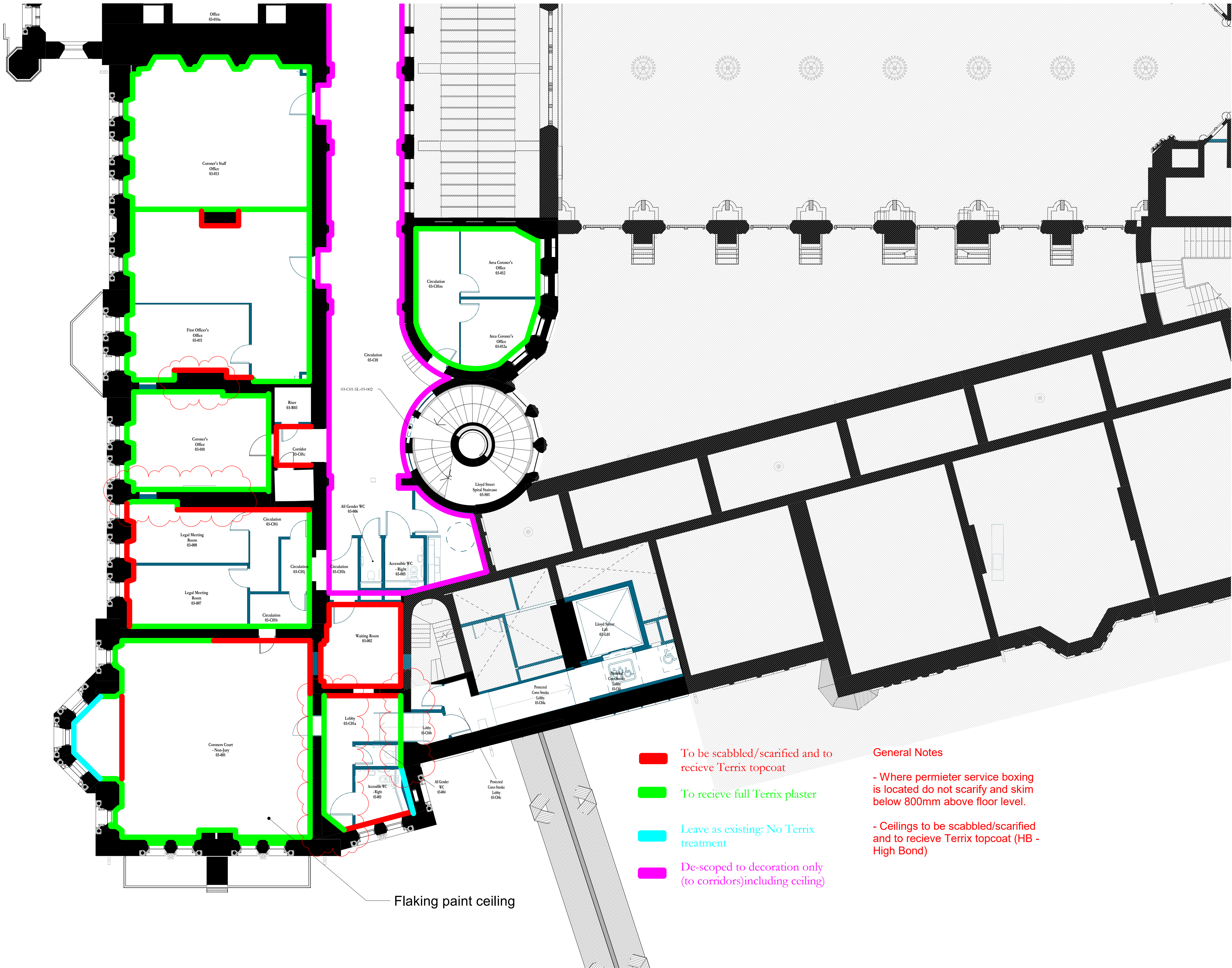
GA PLAN PROPOSED LEVEL 03 - Plaster Removal Plan - 0564 1 : 100
