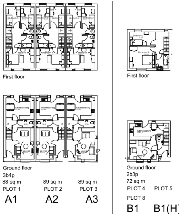
Figure 3 House Types A1, A2, A3 & B1
