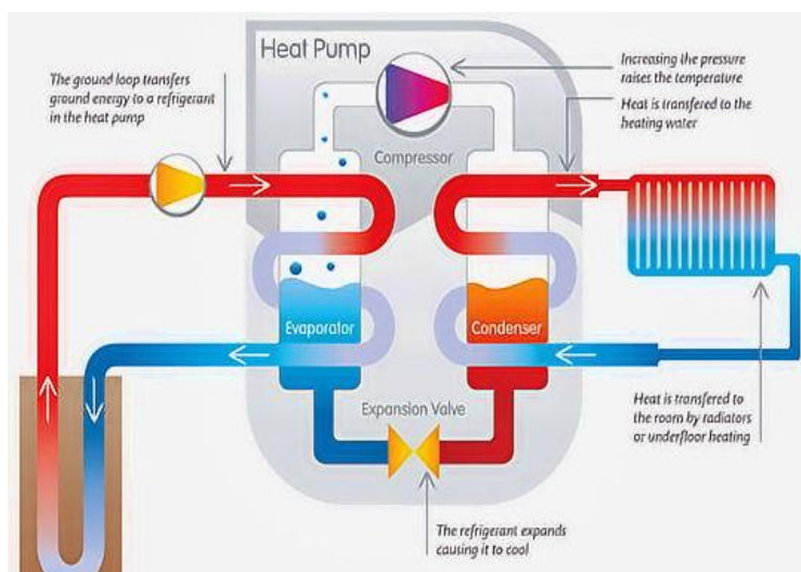
Figure 10 - Principles of a GSHP system
