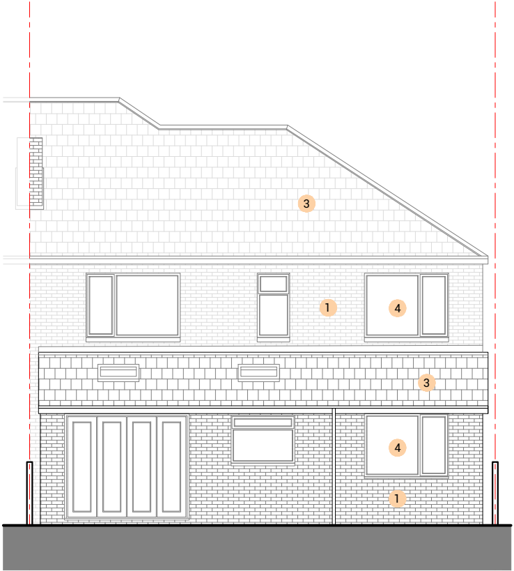
PROPOSED REAR ELEVATION 1:100 @ A3
