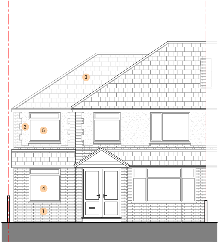
PROPOSED FRONT ELEVATION 1:100 @ A3 0m 1m 3m 5m Key 1 Brickwork to match existing 2 K-rendering to match existing 3 Roof tiles to match existing 4 PVC Window to match existing 5 PVC Window to match existing (Obscure Glazing)
