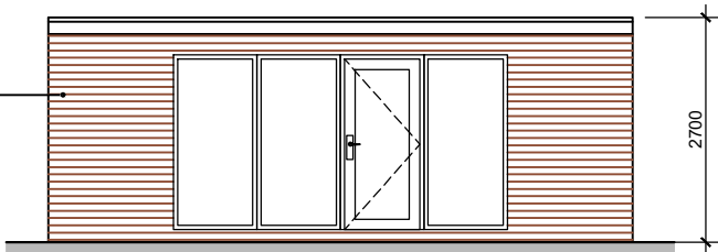
FRONT ELEVATION 1:100
