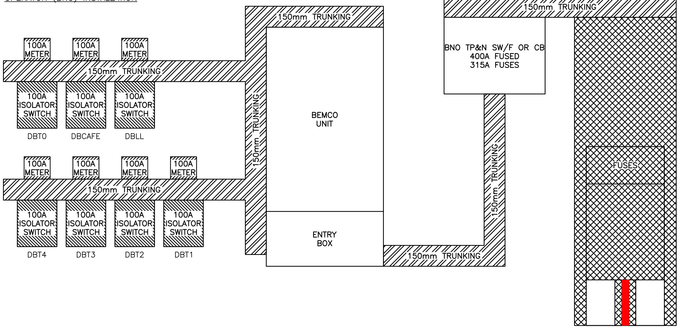
INDICATIVE LAYOUT OF BUILDING NETWORK OPERATOR (BNO) INSTALLATION
