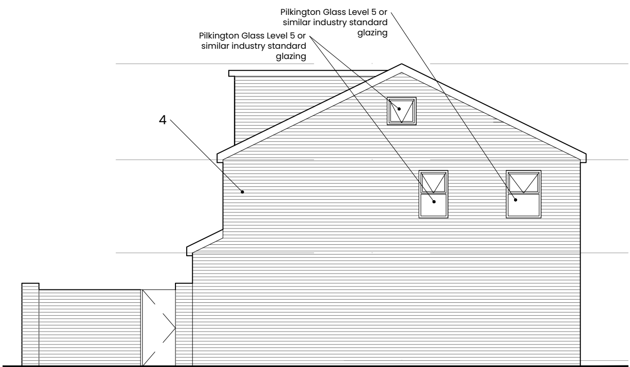
GA Side Elevation along Garlick Street
