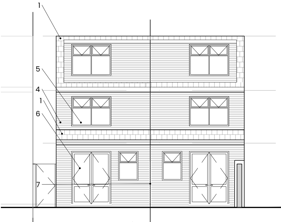
GA Rear Elevation
