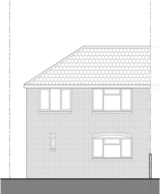
EXISTING REAR ELEVATION 1:100 @ A3 0m 1m 3m 5m
