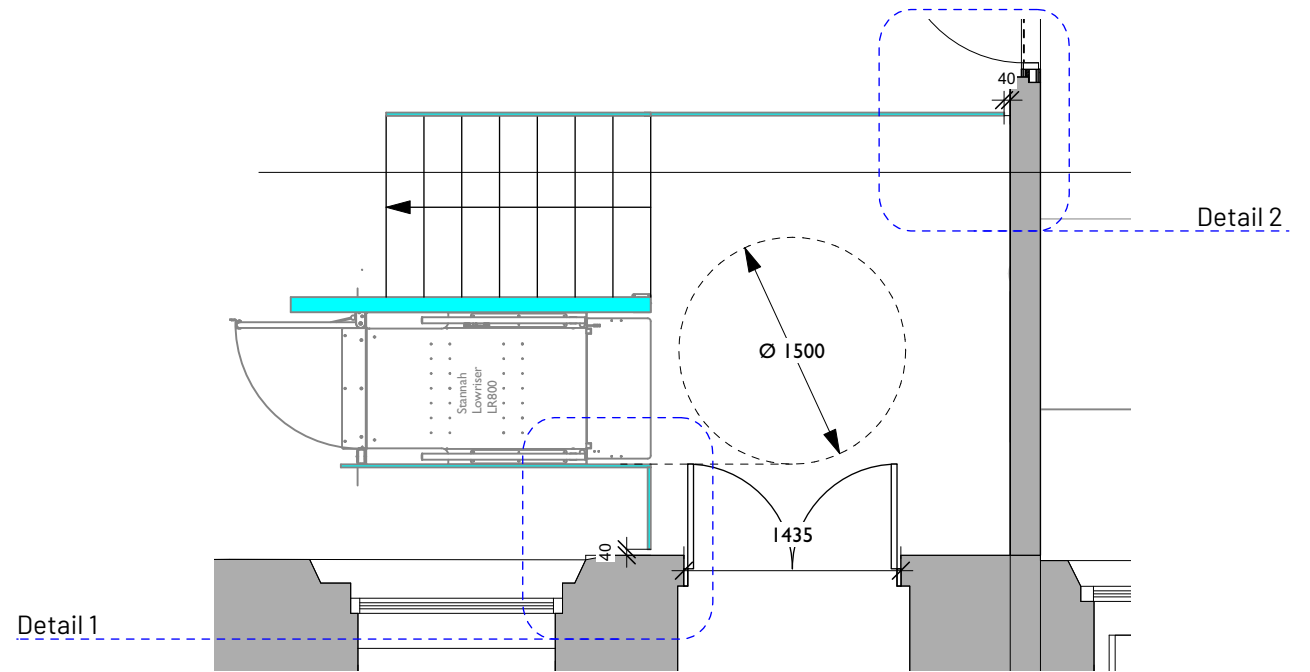
1 Localised Plan Scale: 1:50
