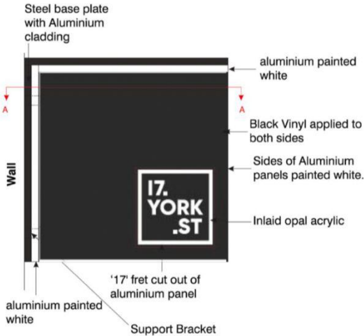
Face (Front Elevation)
