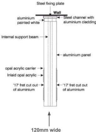
Plan View (Cross section A - A)
