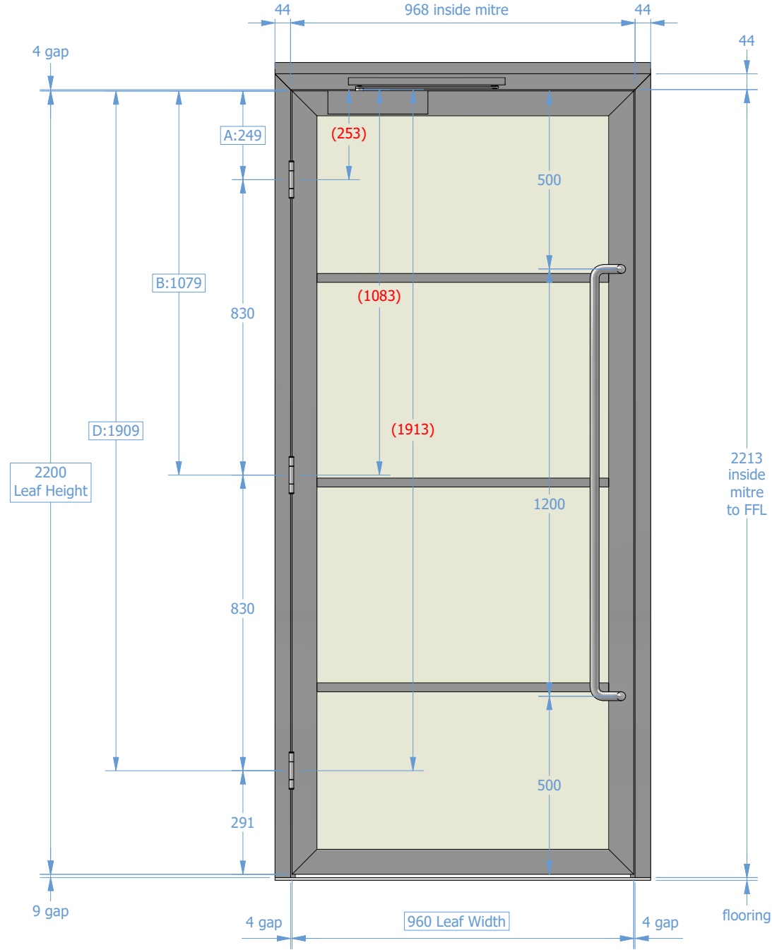
Rear Elevation (TTS) EGI Doorframe Dimensions
