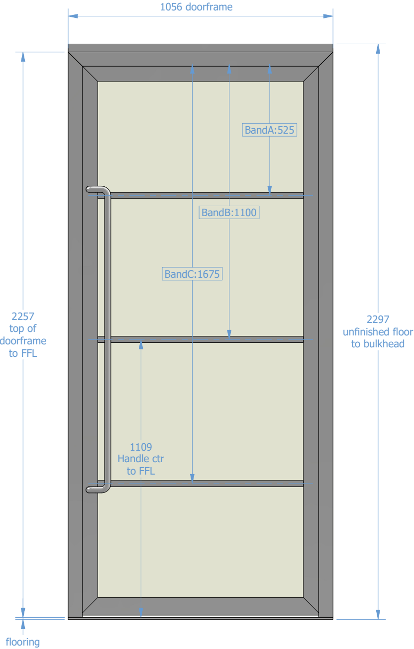
Front Elevation (TTS) EGI Doorframe Dimensions
