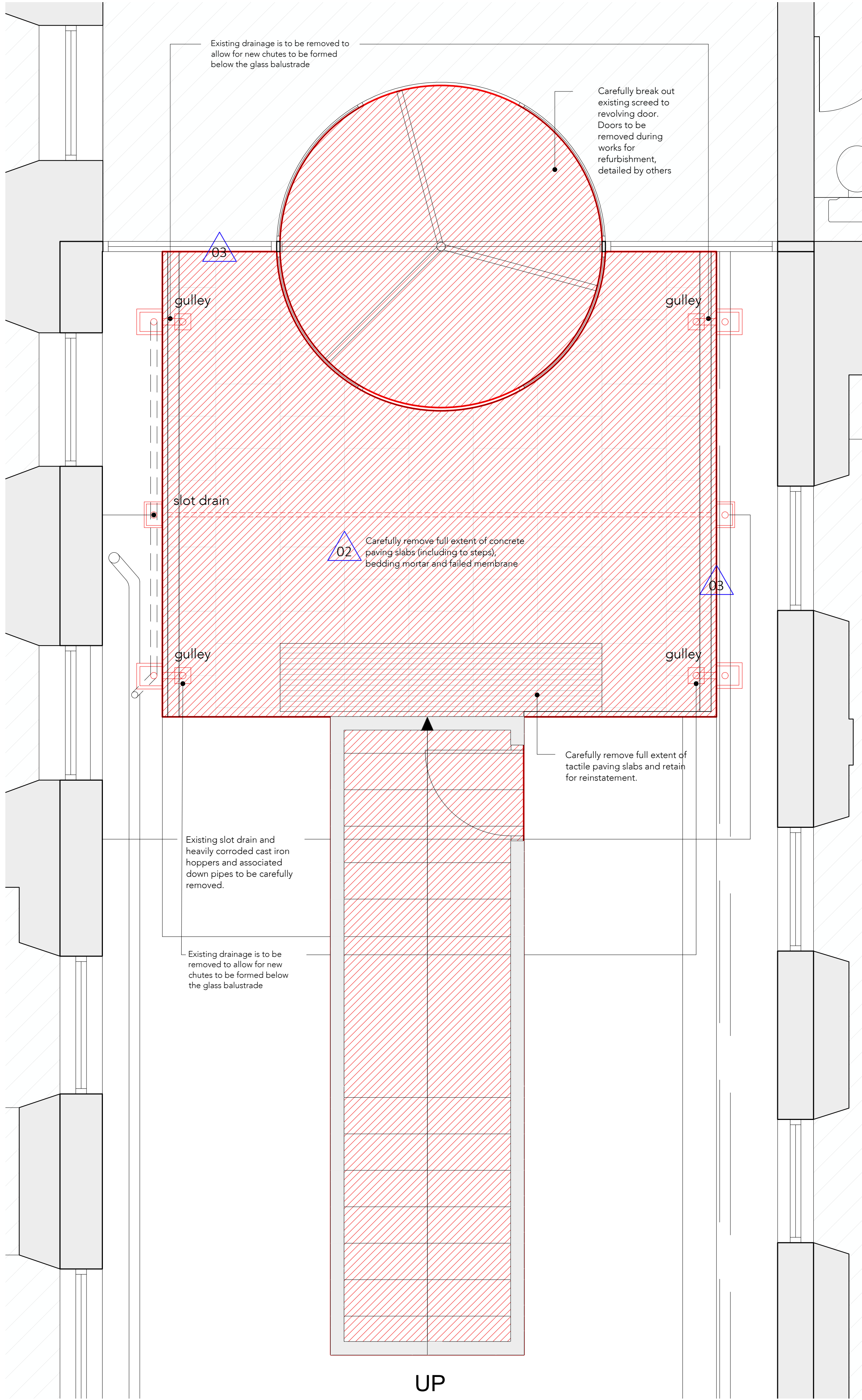
ALTERATIONS PLAN OF ATRIUM ENTRANCE 1:25
