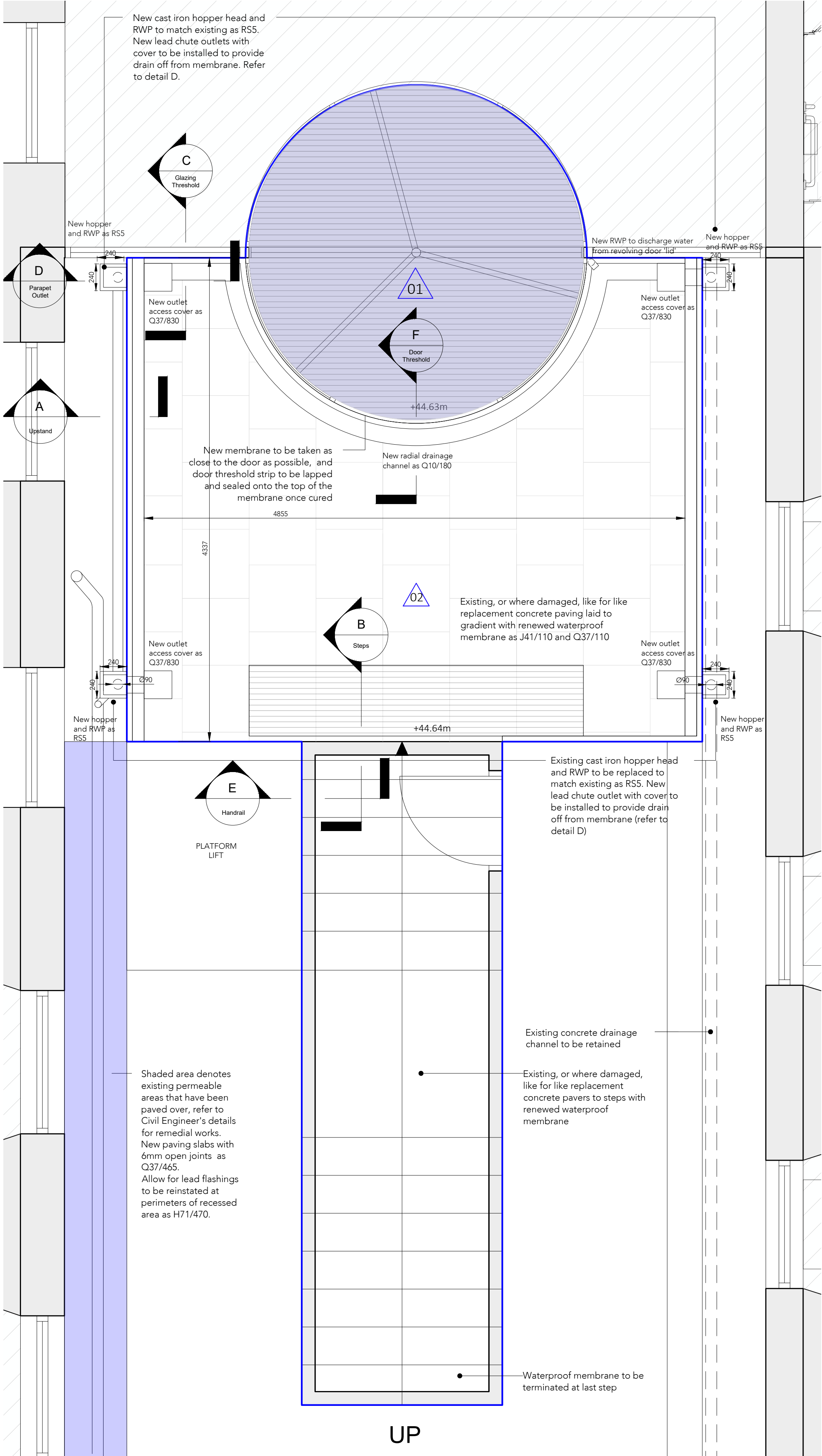
PROPOSED PLAN OF ATRIUM ENTRANCE 1:25
