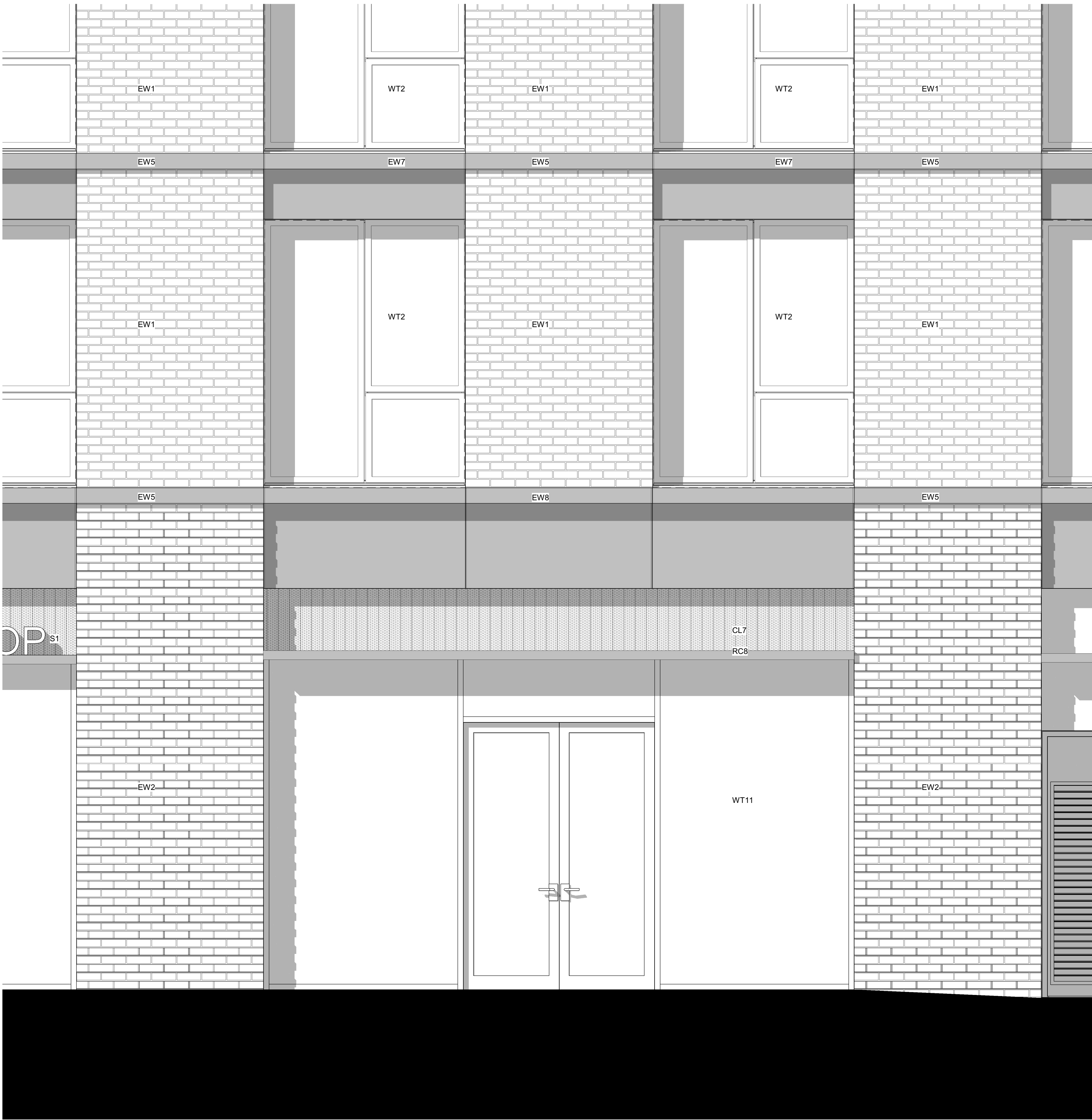
Commercial Bay & Typical Residential Window_Planning 1 : 20
