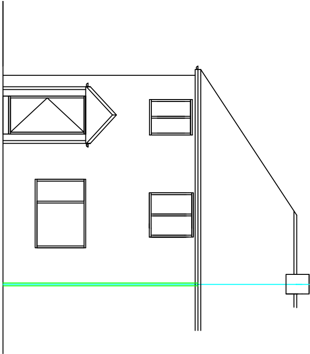
EXISTING FRONT VIEW 1:100
