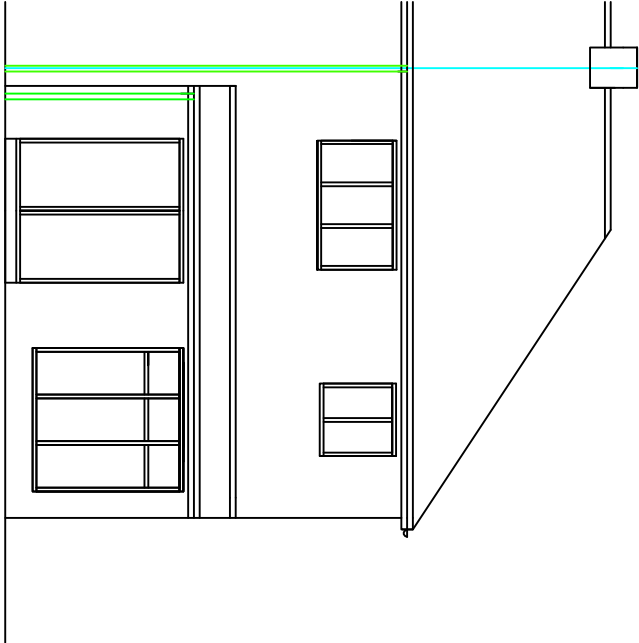
EXISTING REAR VIEW 1:100
