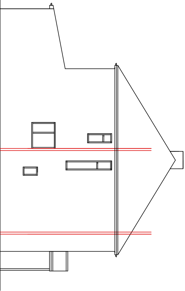
EXISTING SIDE VIEW A 1:100
