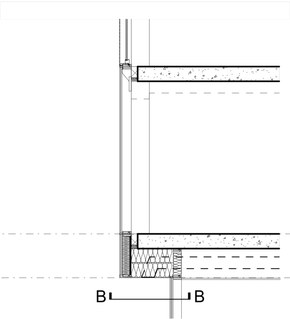
Section AA Scale 1:20 @ A1
