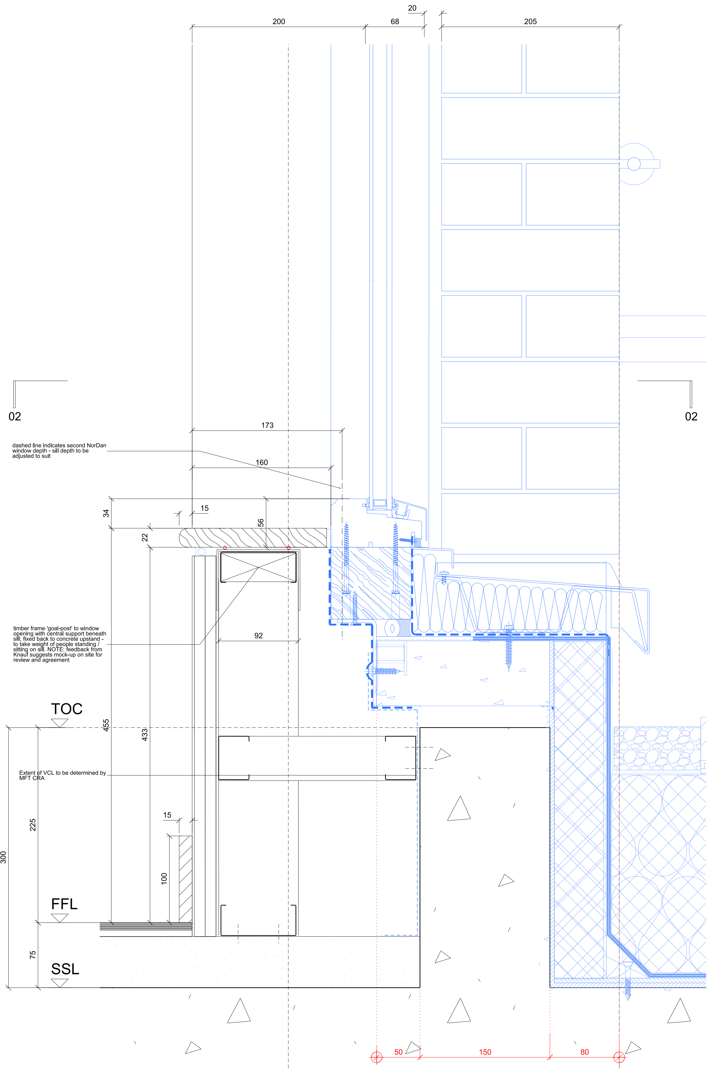
01 Detail Section 1:5 @ A3
