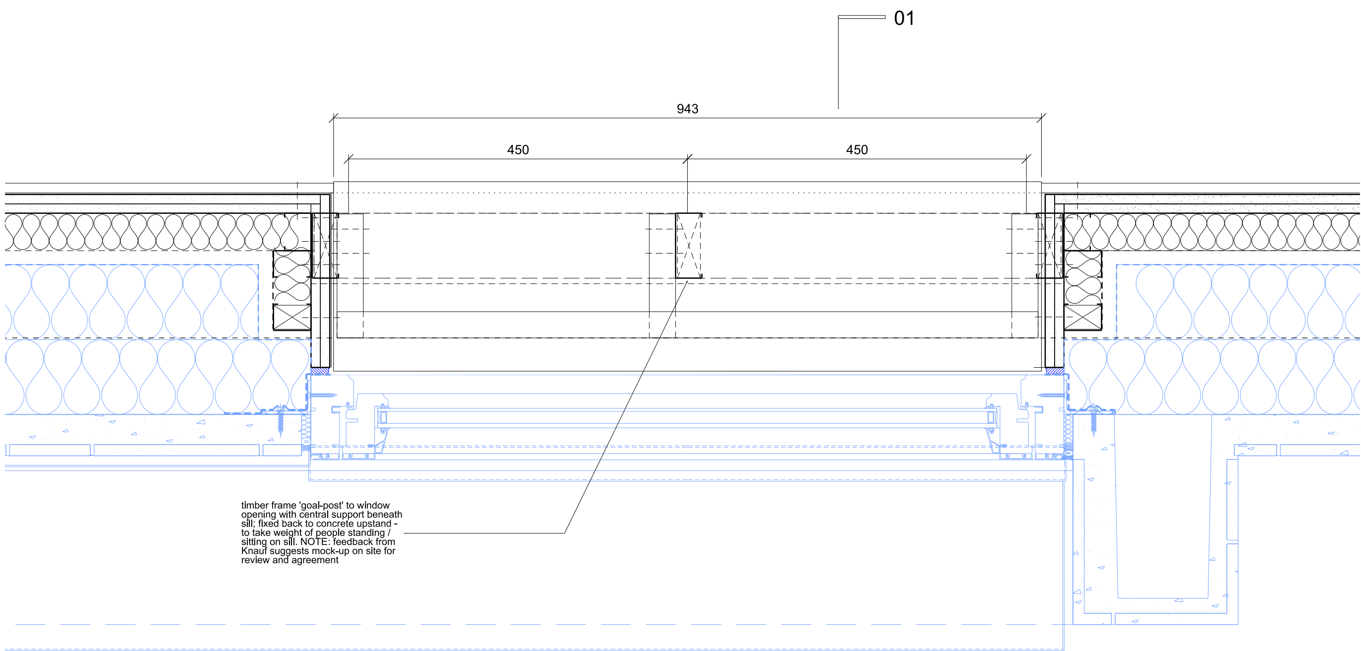
02 Plan Detail 1:10 @ A3
